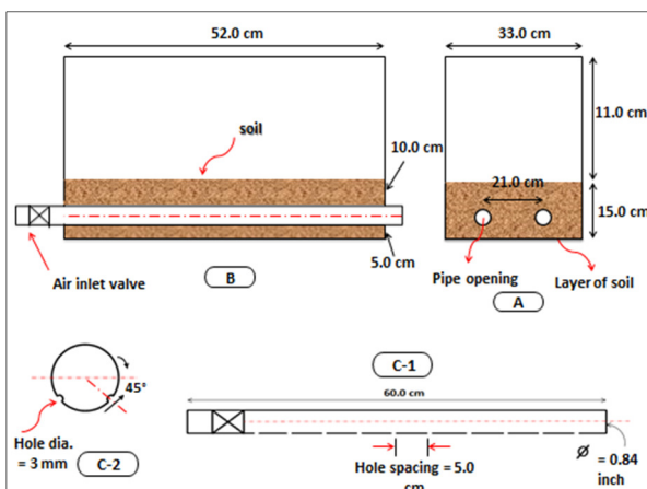
Fig. 2. the dimensions of the stainless steel Biopile system. A: front view B: side view C-1: air supply tube C-2: cross section of air supply tube
