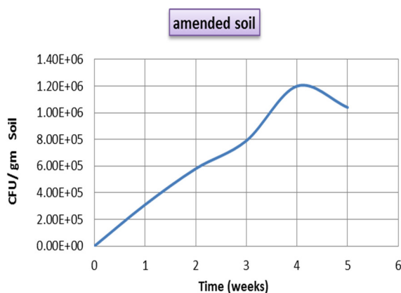
Fig. 5. Changes in counting of diesel-utilizing bacteria for amended soil.
