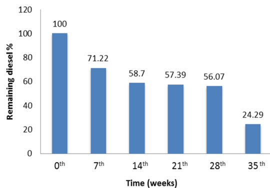
Fig. 3. Percentage of remaining diesel through remediation time in amended soil.
