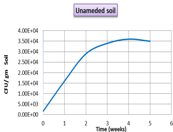
Fig. 6. Changes in counting of diesel-utilizing bacteria for unamended soil (control).
