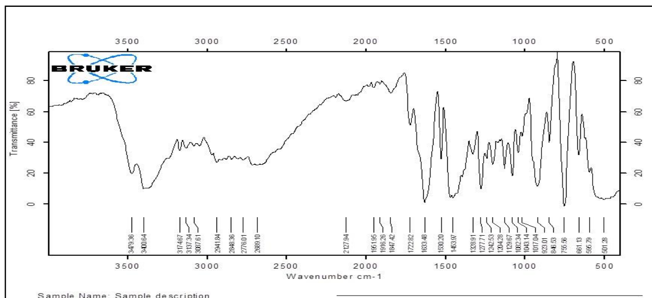
Figure 11. FTIR spectra of (OND and Eudragit RS 100) physical mixture
