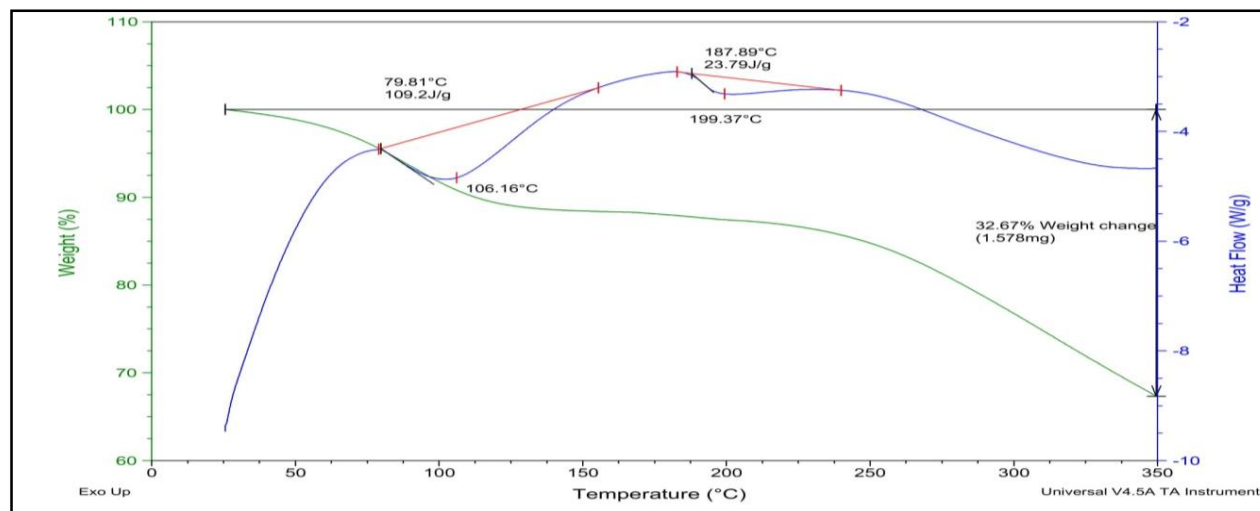
Figure 6. DSC of physical mixture (OND and Eudragit RS 100)
