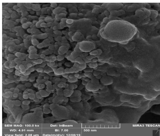
Figure 4. SEM of selected OND nanoparticles (F2)
