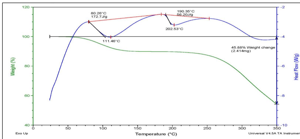
Figure 5. DSC of OND pure drug
