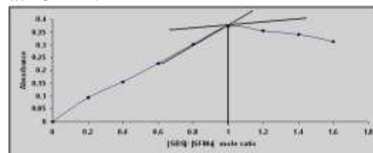
Figure 3. Molar ratio method of sulfamethaxazole.:salbutamol Dye Therefore the formation of the product probably occurs as follows Figure4
