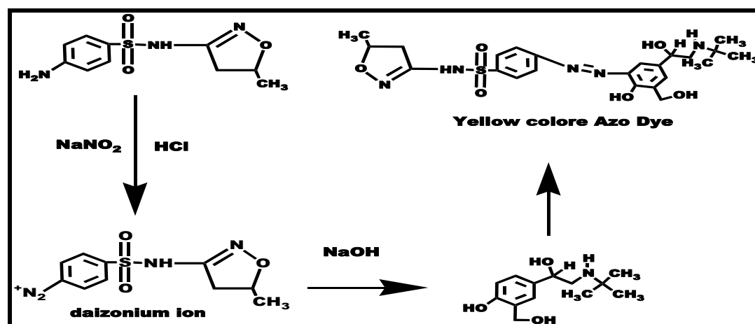
Figure 4 Probable product formation pathway
