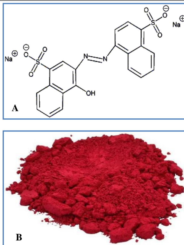
Figure, 1A and B: Chemical structure (A) and powder (B) of Azorubine (3 and 8).
