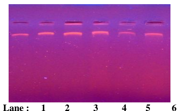
Figure -4- Agarose gel electrophoresis of genomic DNA extracted from control and hyperbilirubinemic neonates with severe G6PD deficiency. (1 -3 bands for normal ; 4- 6 bands for severe G6PD-deficient neonates.
