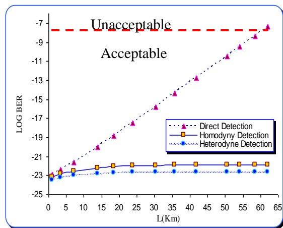
Fig. 5: The variation of the logarithm of BER with the optical fiber length.
