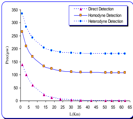
Fig. 2: The variation of received optical power with optical fiber length
