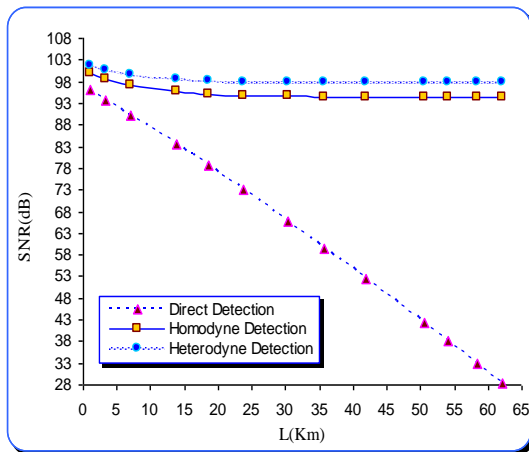
Fig. 4: The variation of SNR with the optical fiber length
