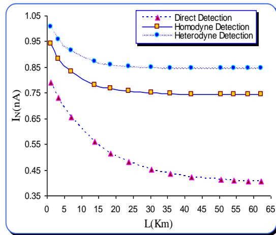
Fig. 3: The variation of the noise current with the optical fiber length.
