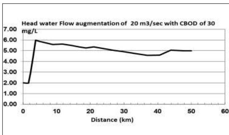
Figure 12: CBOD concentrations along Tigris River in case of control the discharges of point sources as 30 mg/L BOD with flow 20 m 3 /s.
