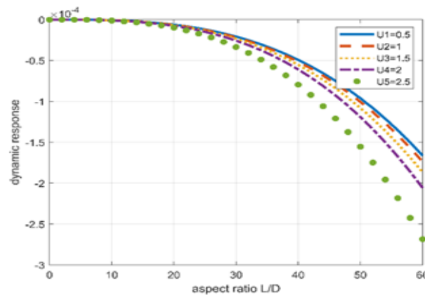
Figure 3: the dynamic response variation vs. aspect ratio for various fluid velocities
