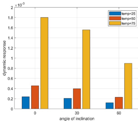
Figure 6: variation of the peak mid-span of dynamic deflection of the pipe with the inclination angles \theta for different temperatures
