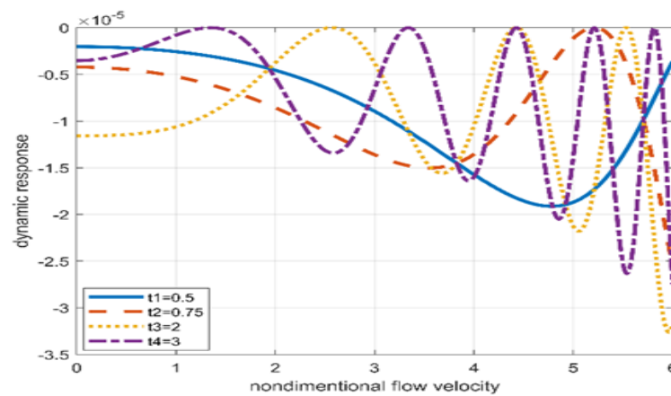
Figure 8: The maximum lateral displacement of the middle point of clamped-clamped pipe conveying fluid versus fluid velocity at different times
