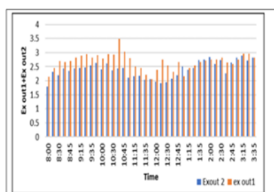
Figure 9: Variation of exergy out along the day for two different heat sink
