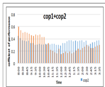
Figure 7: Variation of coefficient of performance (cop) for two different heat sink
