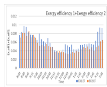
Figure 10: Variation of exergy efficiency through the day for two different types of the heat sink
