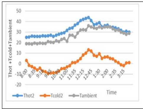
Figure 5: Variation of hot wall air cooler heat sink (HWAC)
