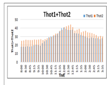
Figure 8: Different temperature hot junction for two heat sinks (HWACHE) and (HWAC)
