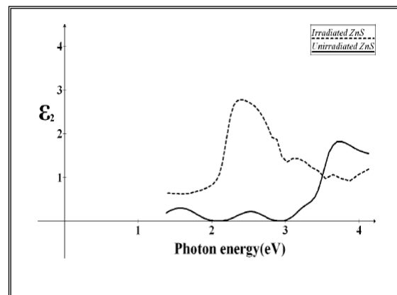
Fig. (5) \epsilon_2 vs. Photon energy.
