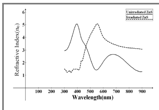
Fig.(2) Refractive Index vs. wavelength.
