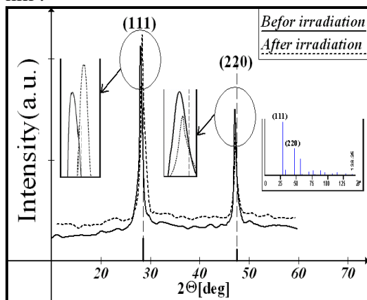
Fig. (1) XRD pattern of irradiated and unirradiated ZnS films.
