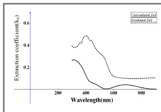
Fig. (3) Extinction coefficient vs. wavelength.
