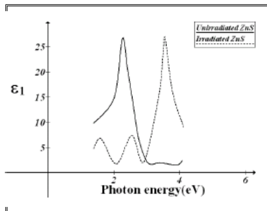
Fig. (4) \epsilon_1 vs. Photon energy.
