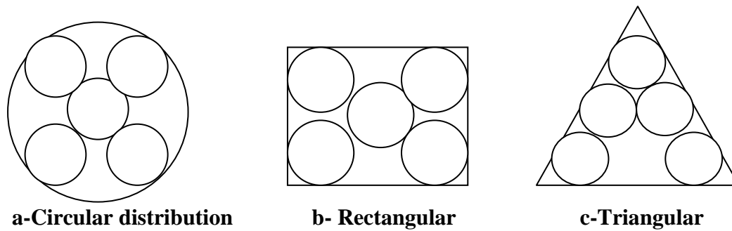
Fig.(1): Three different solar cell distributions in a panel
