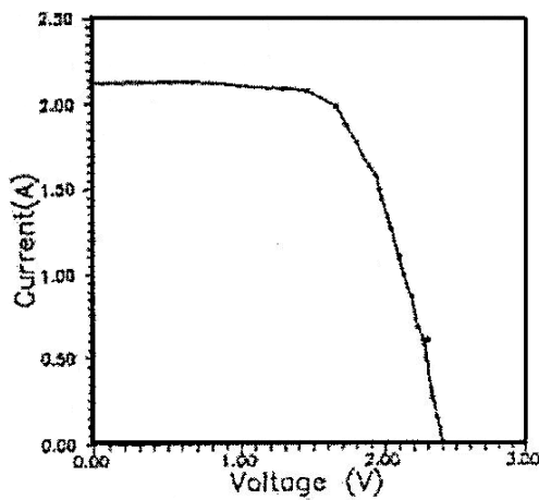
Fig(4-a)-I-V Characteristic of circular panel under the sun .
