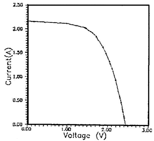
Fig (4-b)-I-V Characteristic of rectangular panel under the sun .
