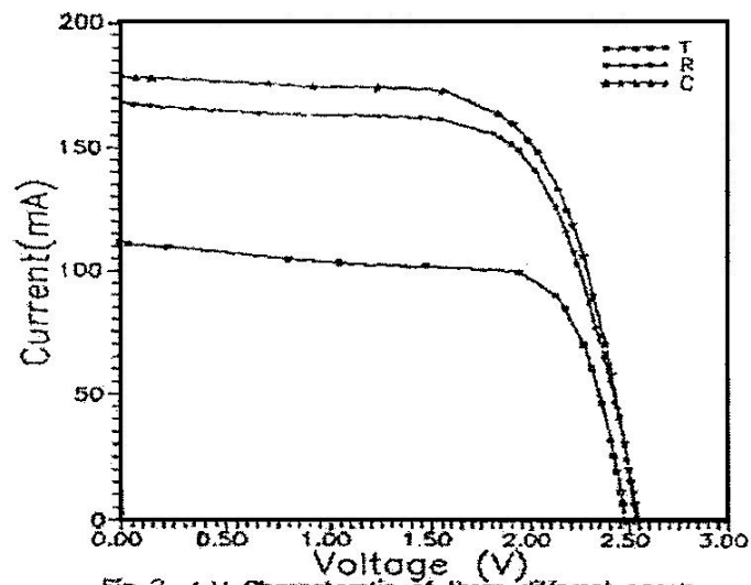
Fig. 3 I-V Characteristic of three different panels measured in laboratory .
