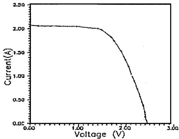
Fig. 4-C I-V Characteristic of triangular panel under the sun.
