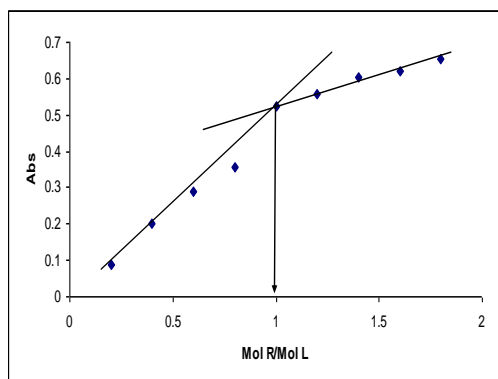
Fig 9: Mole ratio of reagent to sample for the Pd(II) complex .
