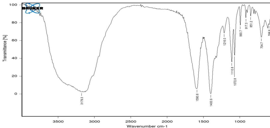
Figure 6. FTIR spectra of raltegravir HME best formulation (Trial 6)
