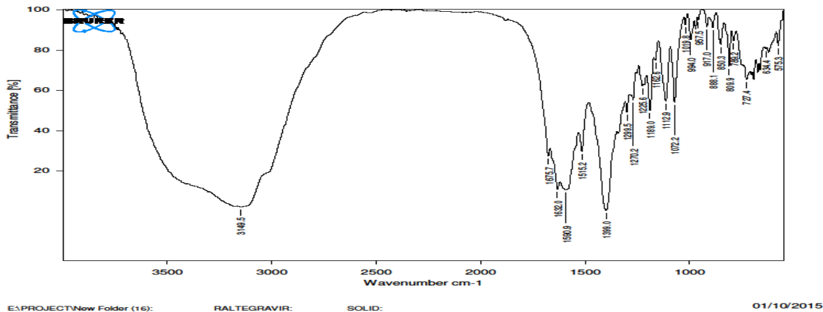
Figure 4. FTIR spectra of raltegravir
