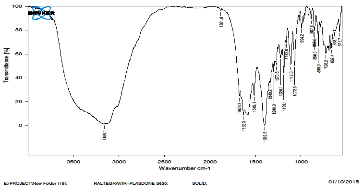
Figure 6. FTIR spectra of raltegravir HME best formulation (Trial 6)
