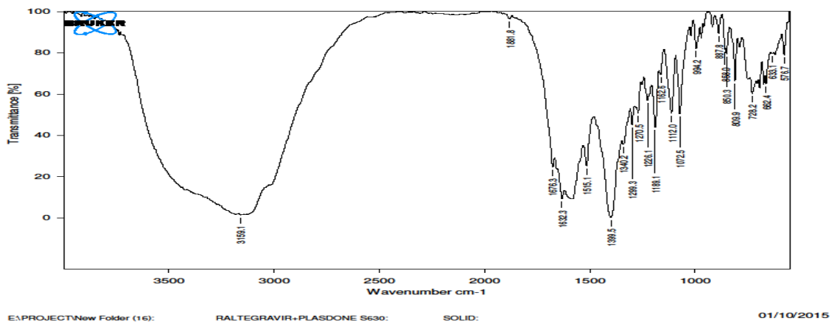
Figure 5. FTIR of physical mixture
