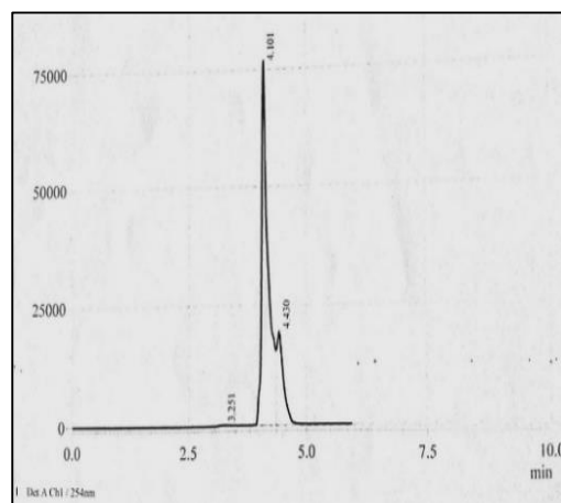
Figure 10 . HPLC chromatogram of isolated alkaloid .
