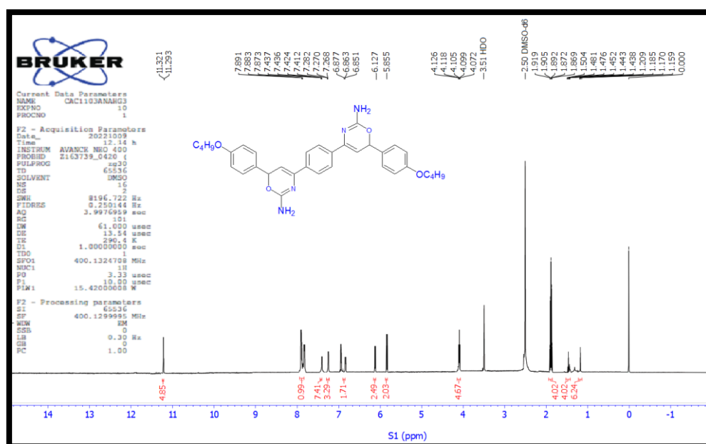
Figure (18): 1 HNMR spectrum of Oxazine (8).
