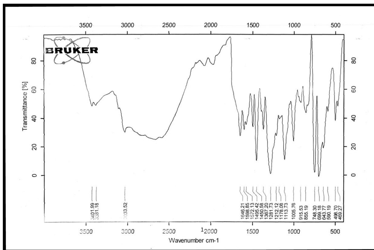
Figure (9): FTIR spectrum of Oxazine 9.
