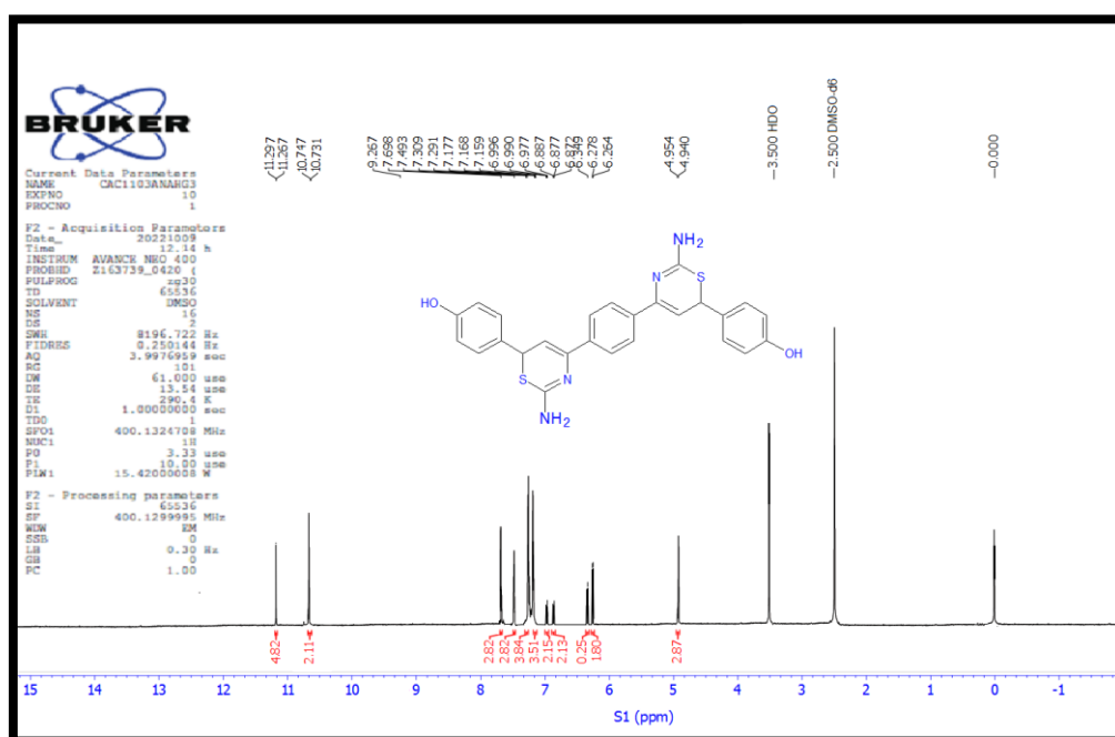
Figure (21): 1 HNMR spectrum of Thiazine (11).
