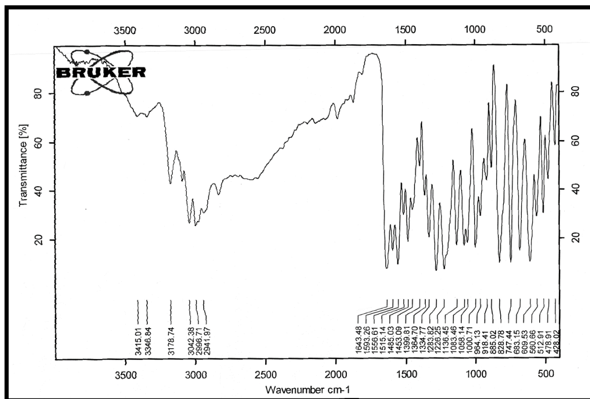
Figure (8): FTIR spectrum of Oxazine 8.
