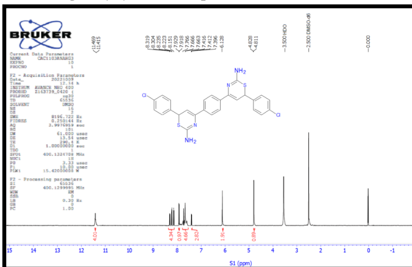
Figure (25): 1 H NMR spectrum of Thiazine (15).
