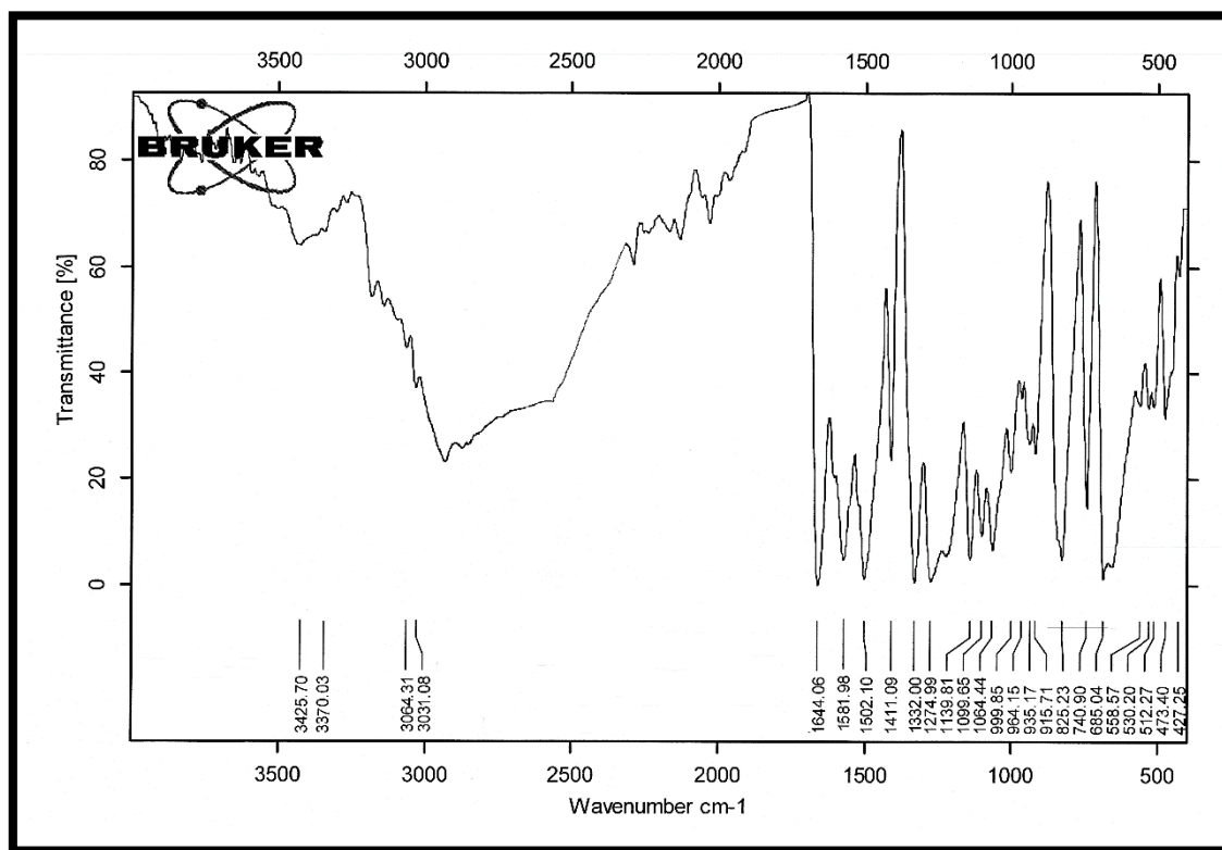
Figure (14): FTIR spectrum of Thiazine 14.
