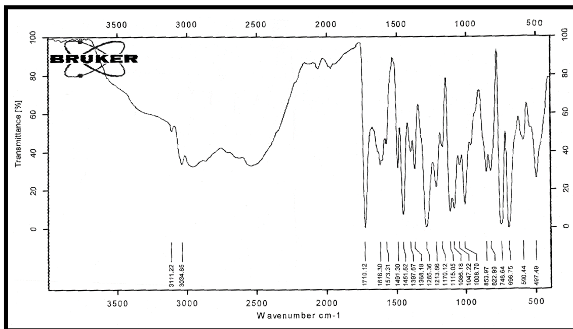
Figure (5): FTIR spectrum of Chalcone 5.
