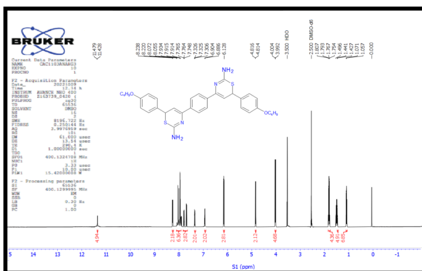
Figure (23): 1 H NMR spectrum of Thiazine (13).
