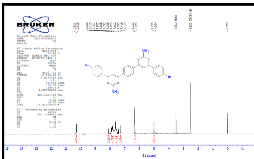
Figure (24): 1 H NMR spectrum of Thiazine (14).
