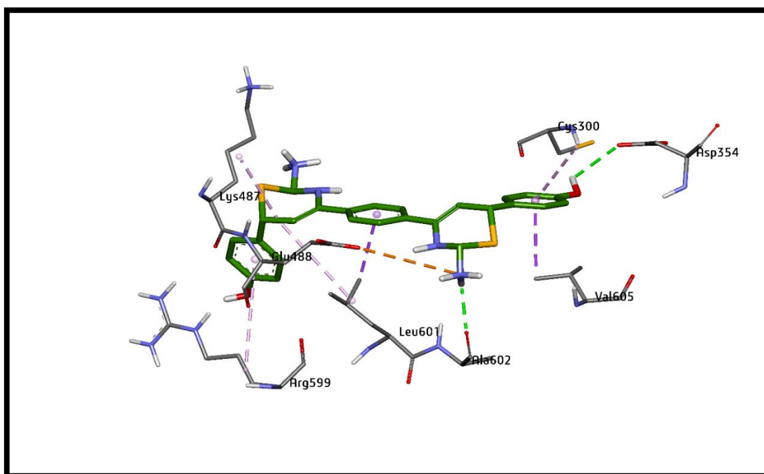
Figure (26): The docking profile of GP6 synthase (PDB ID: 1MOQ) with Thiazine-Hydroxy derivative, a) 3D binding mode.
