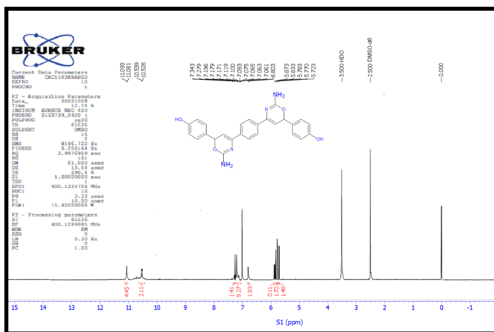
Figure (16): ^1\text{H} NMR spectrum of Oxazine (6).
