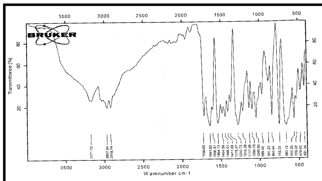
Figure (4): FTIR spectrum of Chalcone 4.
