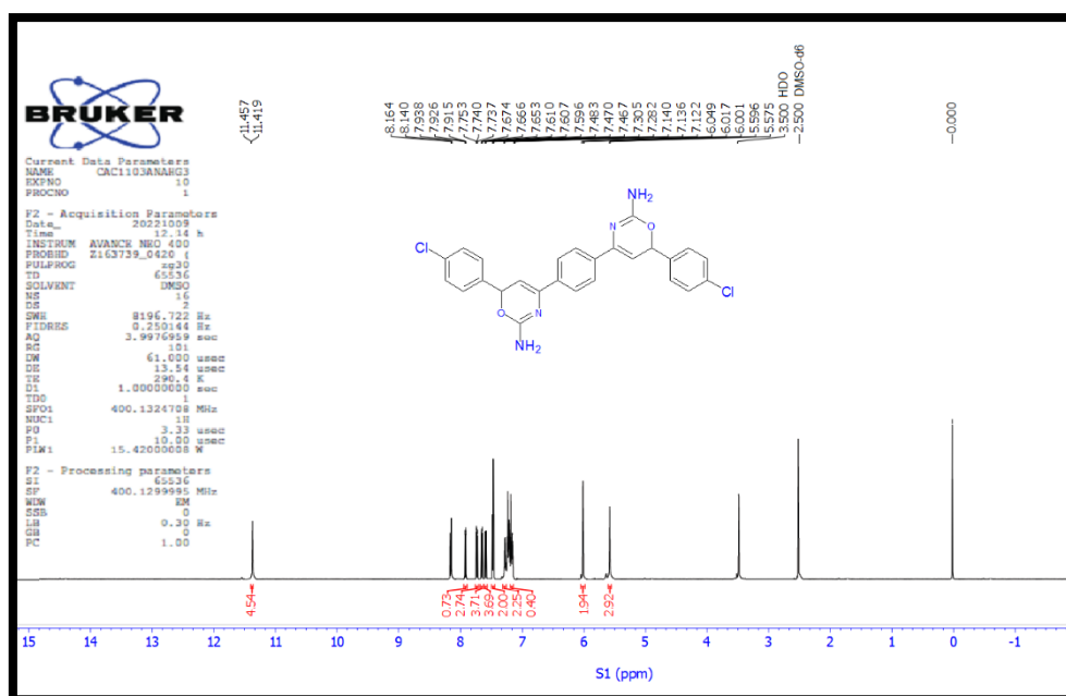
Figure (20): 1 HNMR spectrum of Oxazine (10).
