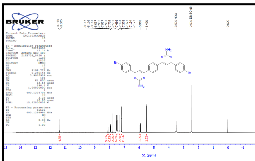
Figure (19): 1 HNMR spectrum of Oxazine (9).
