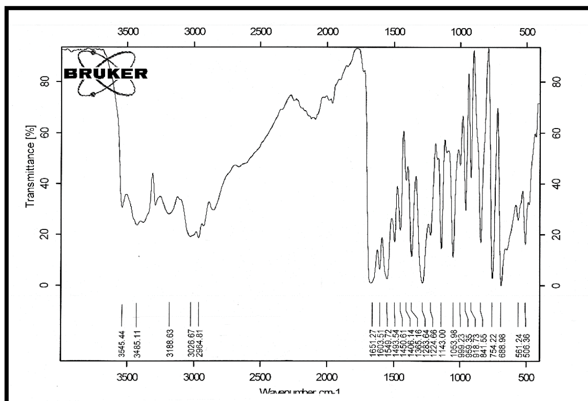
Figure (13): FTIR spectrum of Thiazine 13.
