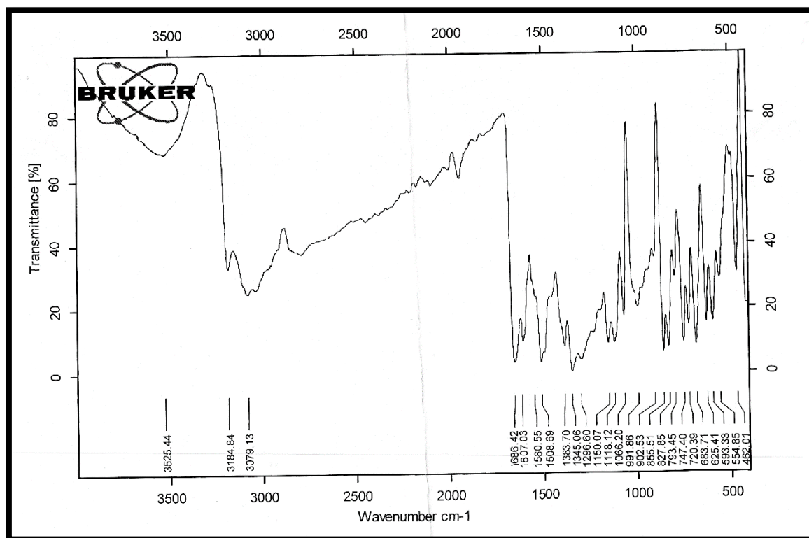
Figure (1): FTIR spectrum of Chalcone 1.
