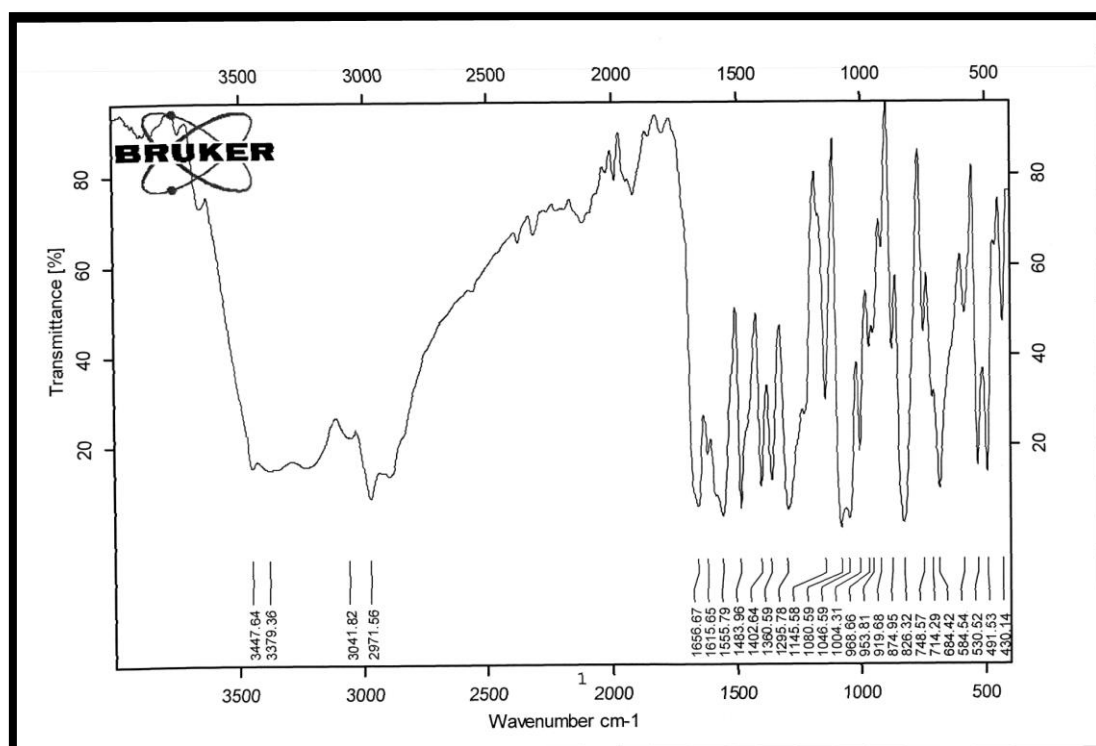
Figure (6): FTIR spectrum of Oxazine 6.
