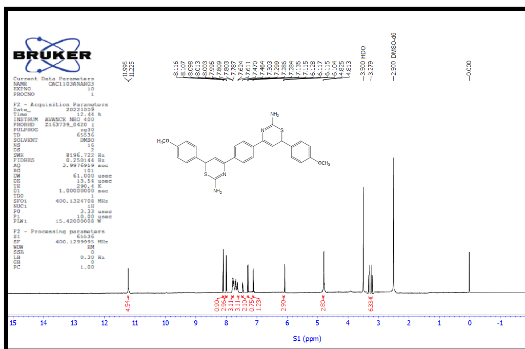
Figure (22): 1 HNMR spectrum of Thiazine (12).
