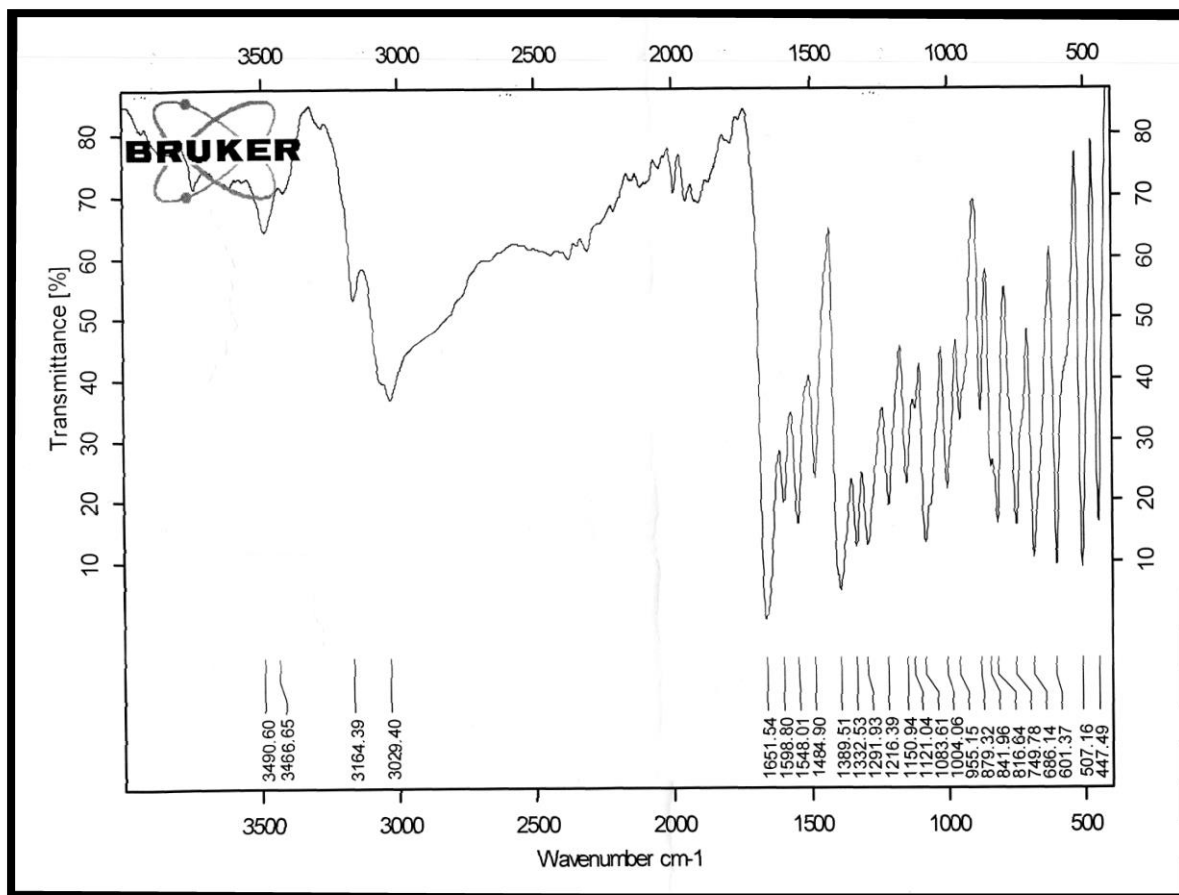
Figure (15): FTIR spectrum of Thiazine 15.
