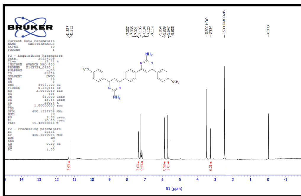
Figure (17): 1 HNMR spectrum of Oxazine (7).
