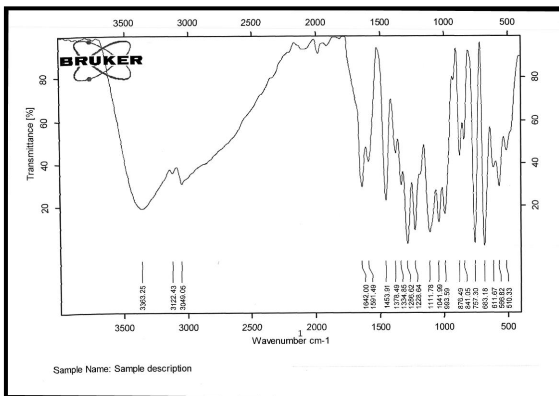
Figure (11): FTIR spectrum of Thiazine 11.
