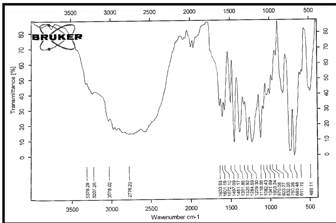
Figure (12): FTIR spectrum of Thiazine 12.
