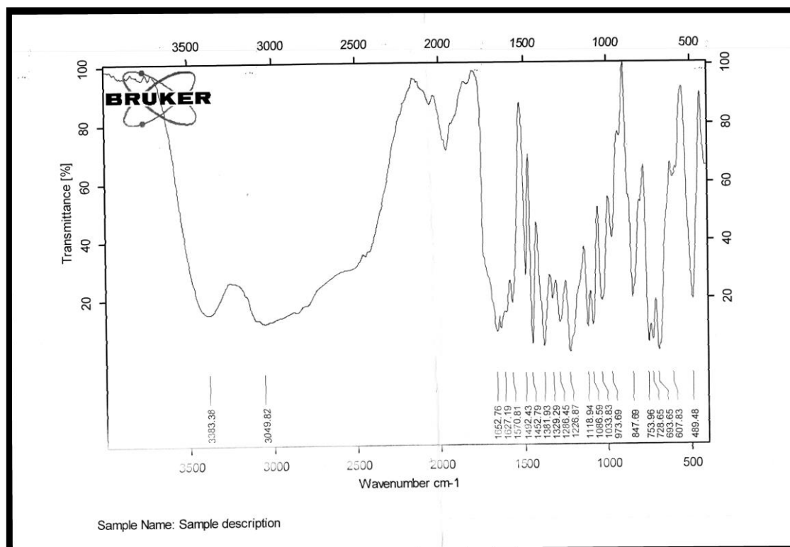
Figure (6): FTIR spectrum of Oxazine 6.
