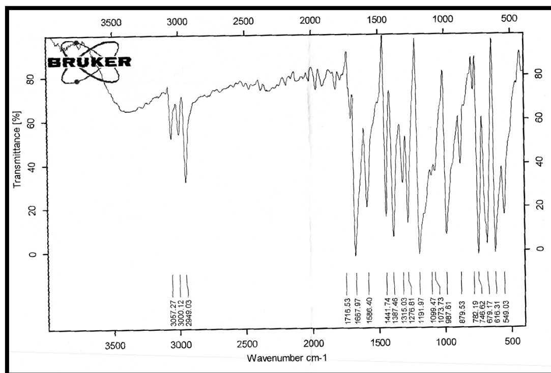
Figure (3): FTIR spectrum of Chalcone 3.
