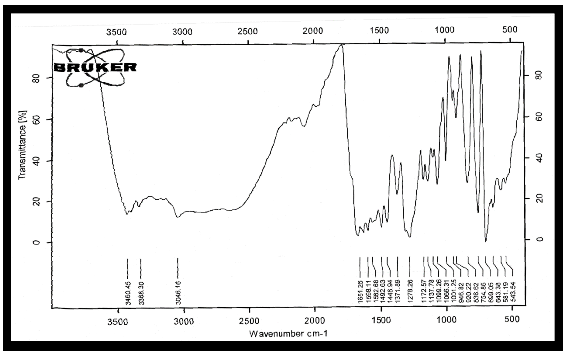
Figure (10): FTIR spectrum of Oxazine 10.
