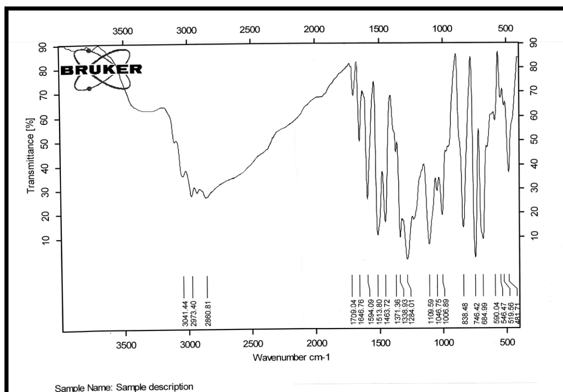
Figure (2): FTIR spectrum of Chalcone 2.
