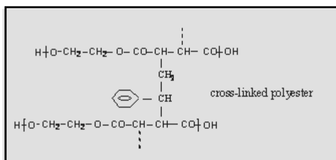
Figure (1): Unsaturated polyester structure.
