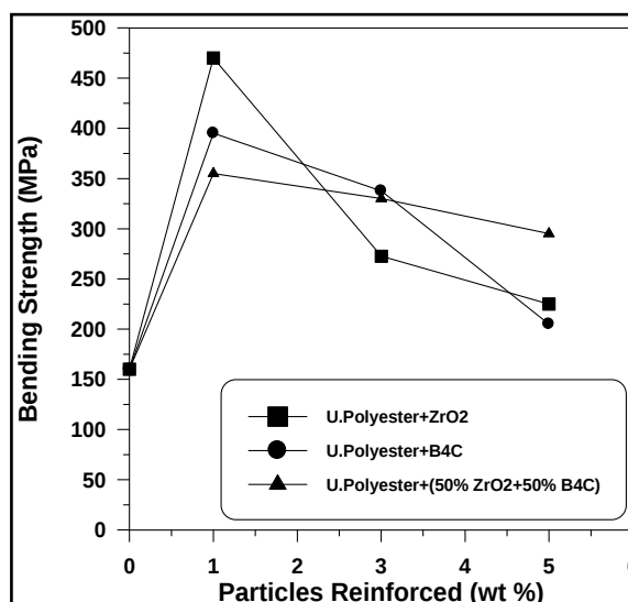
Figure (4) Effect of particle contents on bending strength.
