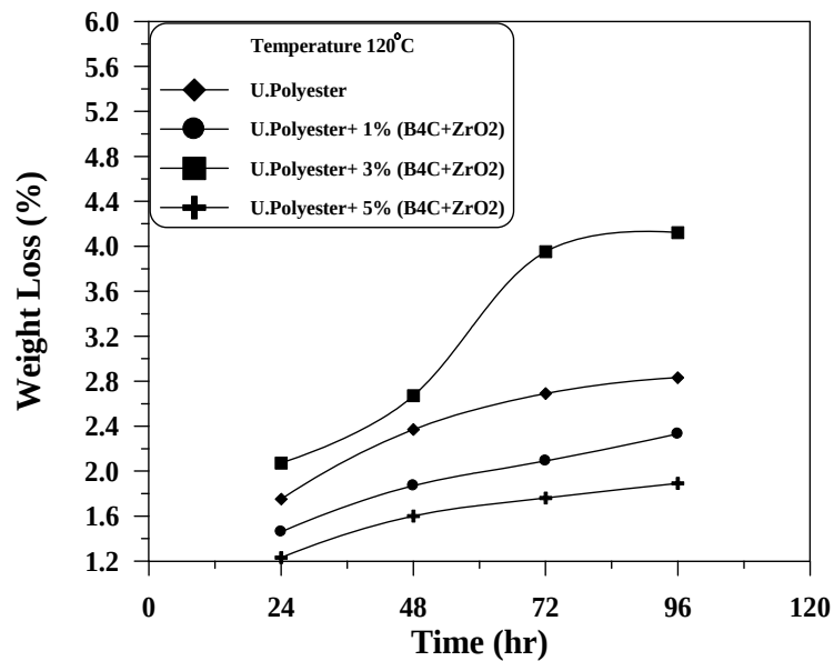
Figure (9) Effect of time exposure to heat on polymer weight loss.
