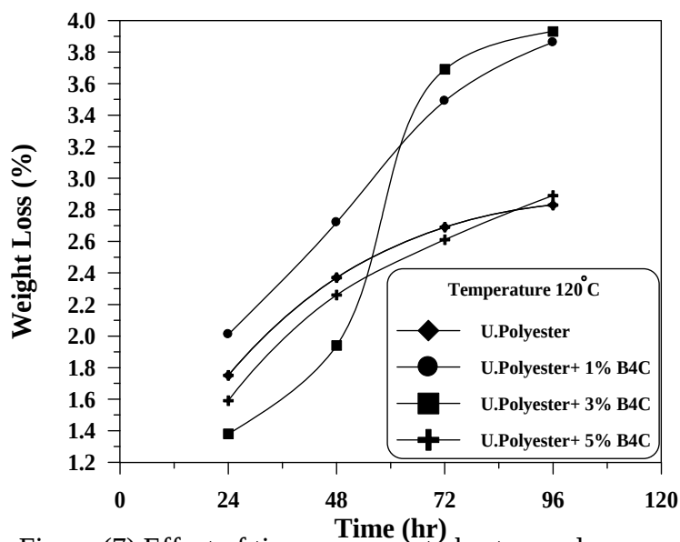
Figure (7) Effect of time exposure to heat on polymer weight loss.
