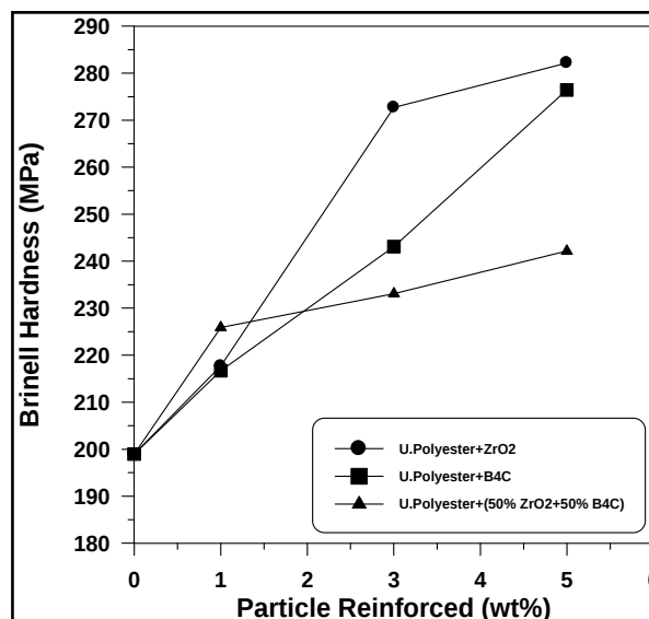
Figure (3) Effect of Particle contents on Hardness.
