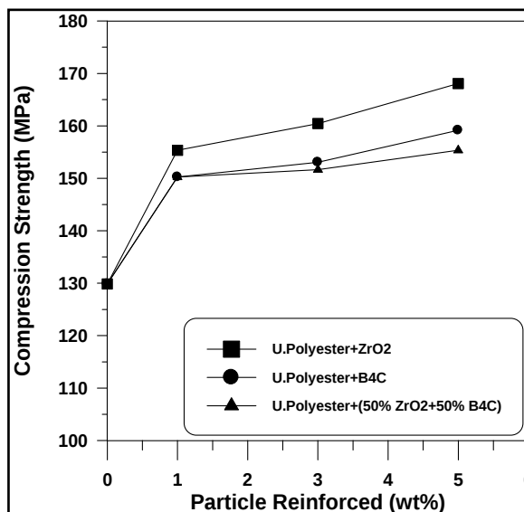
Figure (5) Effect of Particle contents on compression strength.
