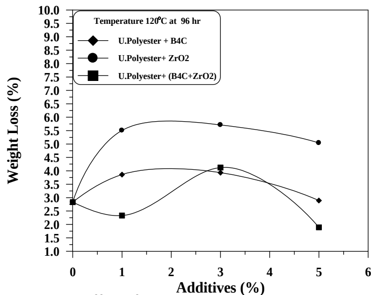
Figure (10) Effect of time additives percent on polymer weight loss.
