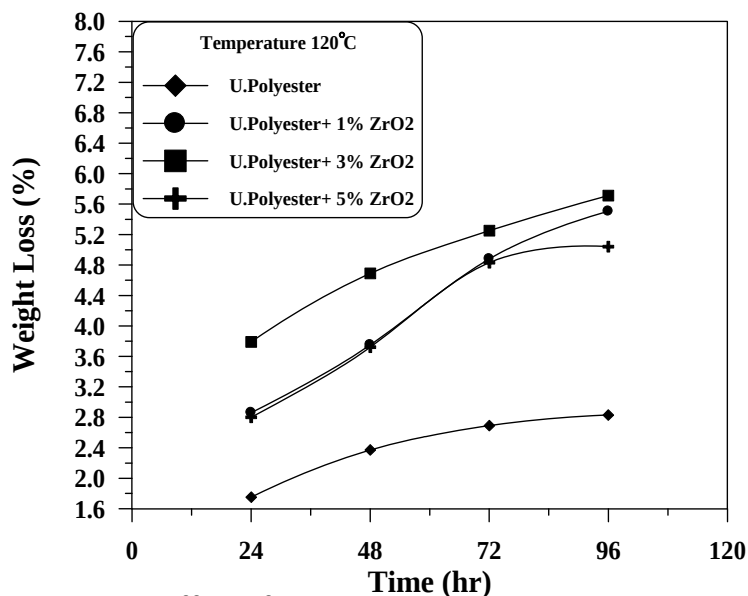
Figure (8) Effect of time exposure to heat on polymer weight loss.
