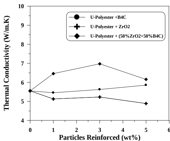
Figure (6) Effect of Particle contents on thermal conductivity.
