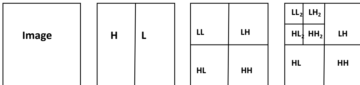
Fig. (1): Two dimensional wavelet transformation of an image
