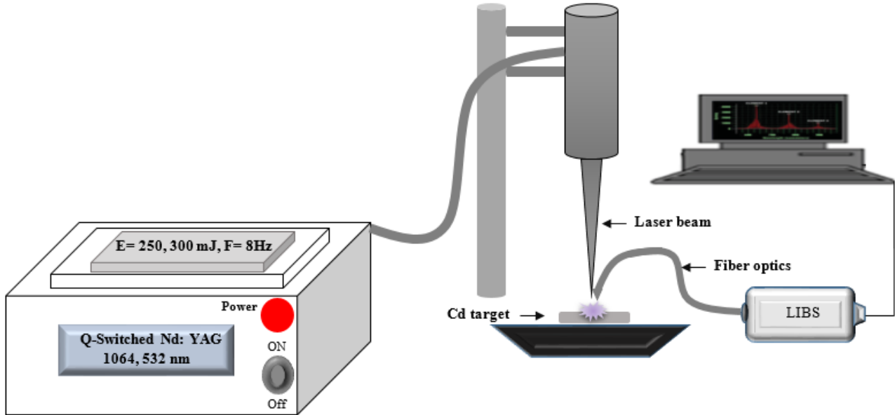
Figure 1. Block diagram of the experimental setup of the LIBS system
