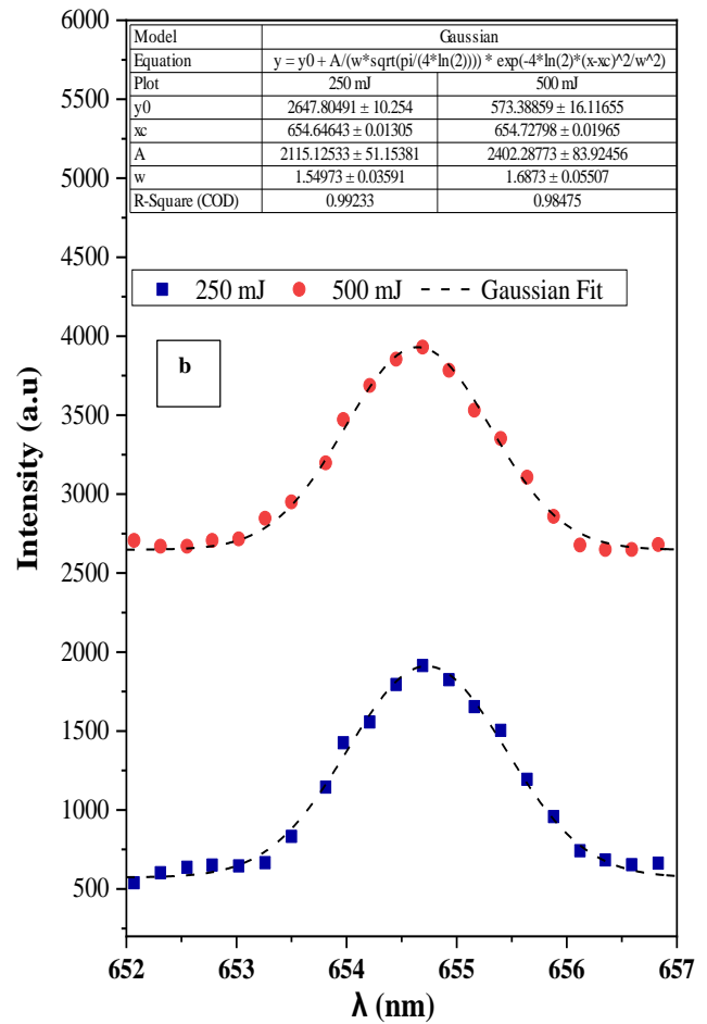
Figure 6. Gaussian fitting of the (a) N (II) for FHG, and (b) (Cd II) for SHG transition for a variety of energies.
