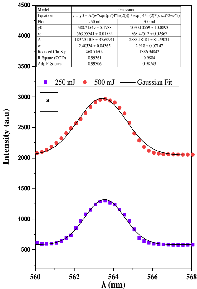
Figure 6. Gaussian fitting of the (a) N (II) for FHG, and (b) (Cd II) for SHG transition for a variety of energies.
