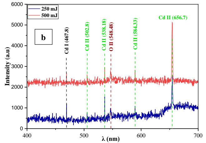
Figure 2. Displays the emission spectra of Cadmium plasma inside a distinct window, encompassing the spectral ranges of 400 to 700 nm. These spectra are generated by the utilization of the (a) first harmonic 1064 nm and (b) second harmonic 532 nm of the laser for different laser energy.
