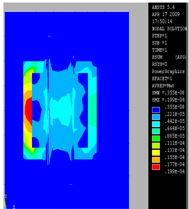
Fig. (15): Nodal Display of Magnetic Flux Density Electromagnetic Casting Process (380/190 A, 50 Hz)
