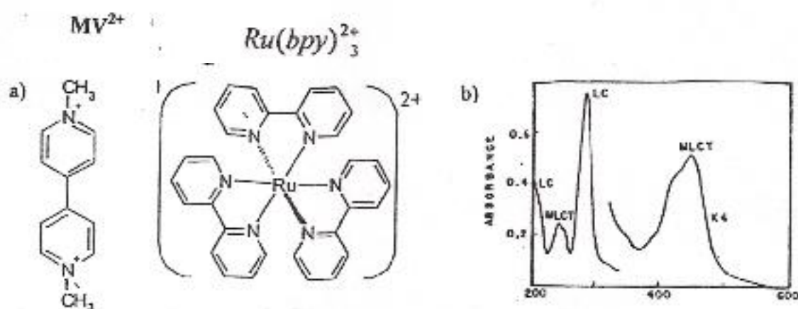
Fig.(1) a - The structure of Ru(bpy)_3^{2+} and MV^{2+} b- absorption spectrum for Ru(bpy)_3^{2+}
