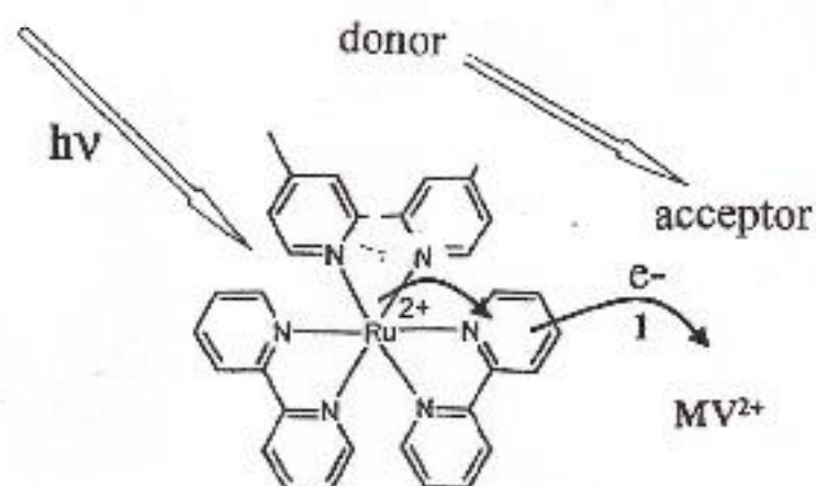
Fig.(2) Electron transfer from the excited state of Ru(II)^* to MV^{2+}
