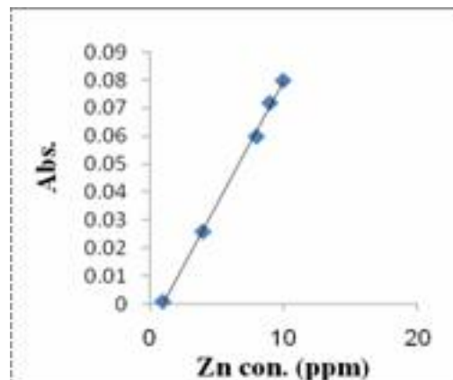
Fig.(4): Calibration curve for zinc
