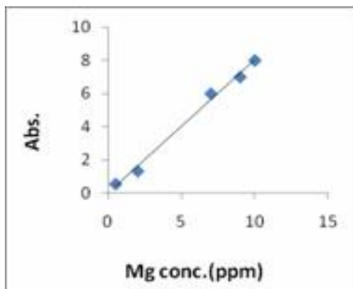
Fig. (3): Calibration curve for magnesium
