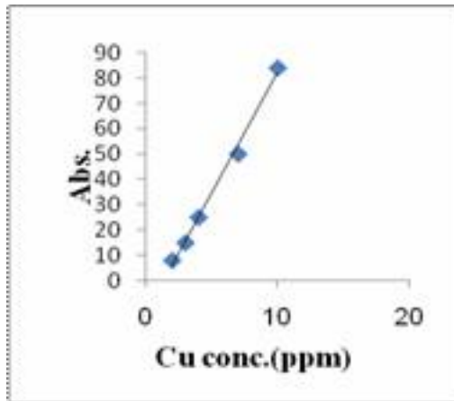
Fig. (1): Calibration curve for copper
