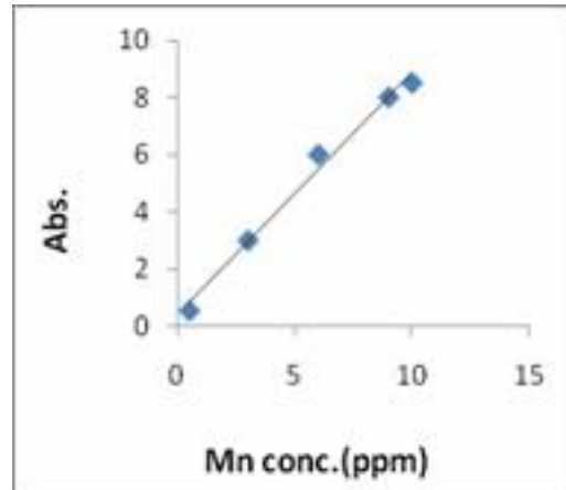
Fig.(2): Calibration curve for manganese
