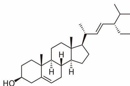
Fig (1): Stigmasterol structure
