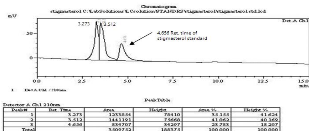
Fig (6): HPLC Chromatogram of stigmasterol standard.
