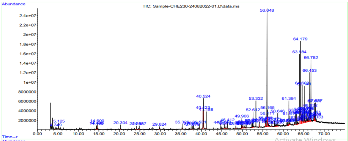
Fig (3): GC-MS chromatogram of hexane extract of arial part
