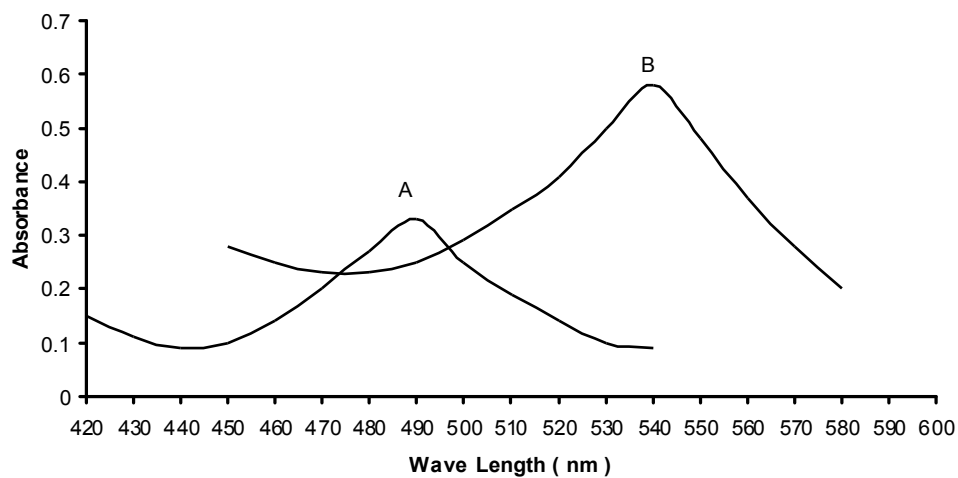
Fig (1) : Absorbance Spectra
