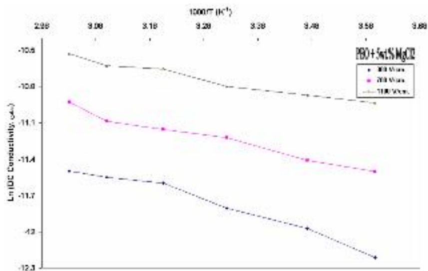
Fig. (2): Natural Logarithm of DC-Conductivity vs. 1000/T for 5wt.% MgCl₂ (at different d.c. polarizing fields)
