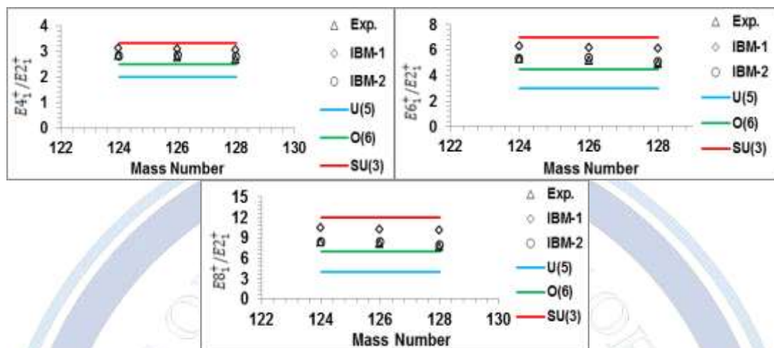
Figure 1: The experimental [29-36], theoretical and standard [15] energy ratios ( E4_1^+/E2_1^+ , E6_1^+/E2_1^+ , and E8_1^+/E2_1^+ ) respectively as a function of mass numbers for even-even ^{124-128}\text{Ba} isotopes.
