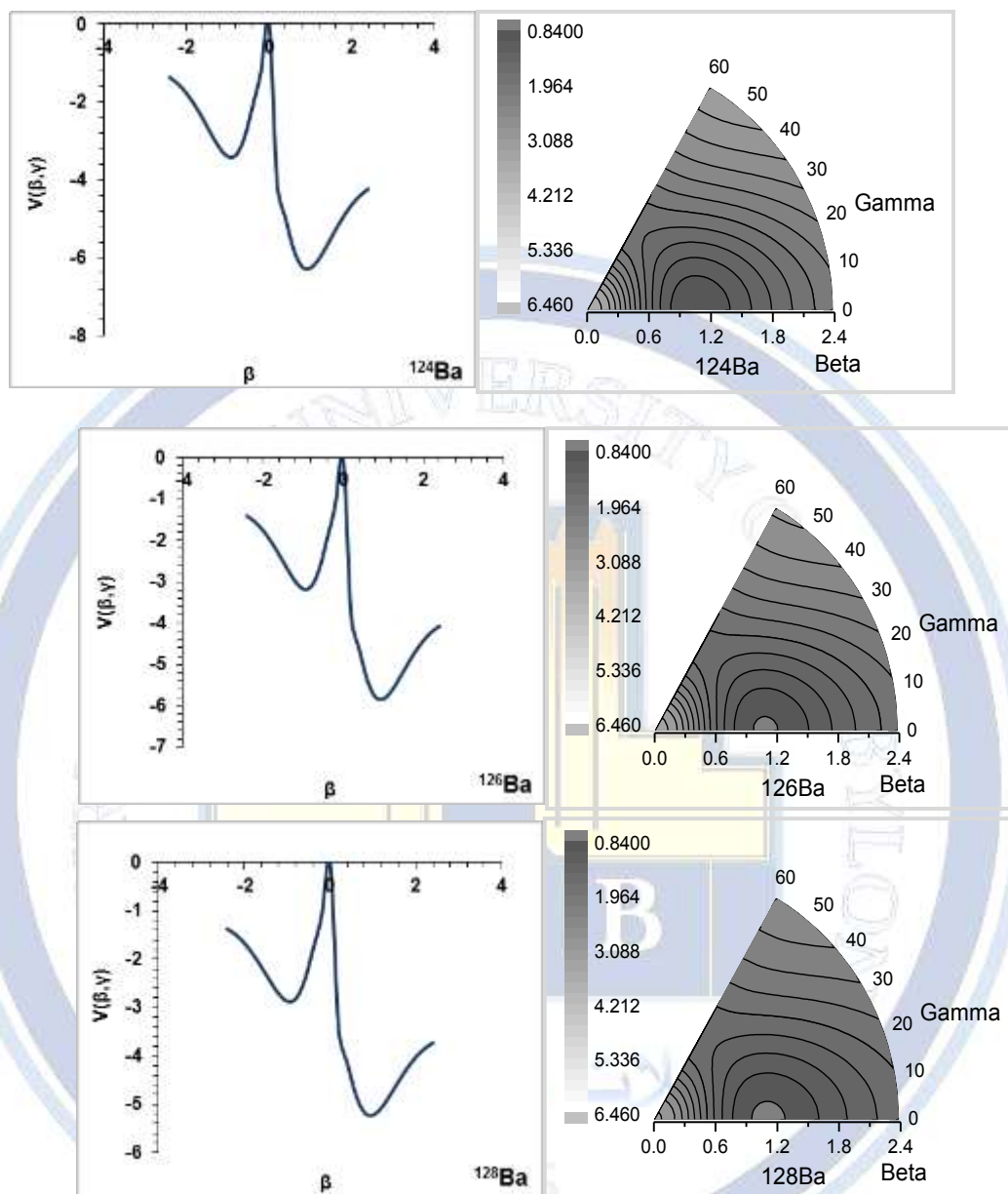
Figure 6: Potential energy surface as a function to \beta with contour diagrams for even-even ^{124-128}\text{Ba} isotopes
