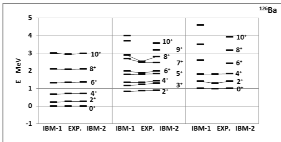
Figure 3: Comparison between experimental [35] and calculated energy levels for ^{126}\text{Ba} isotope.
