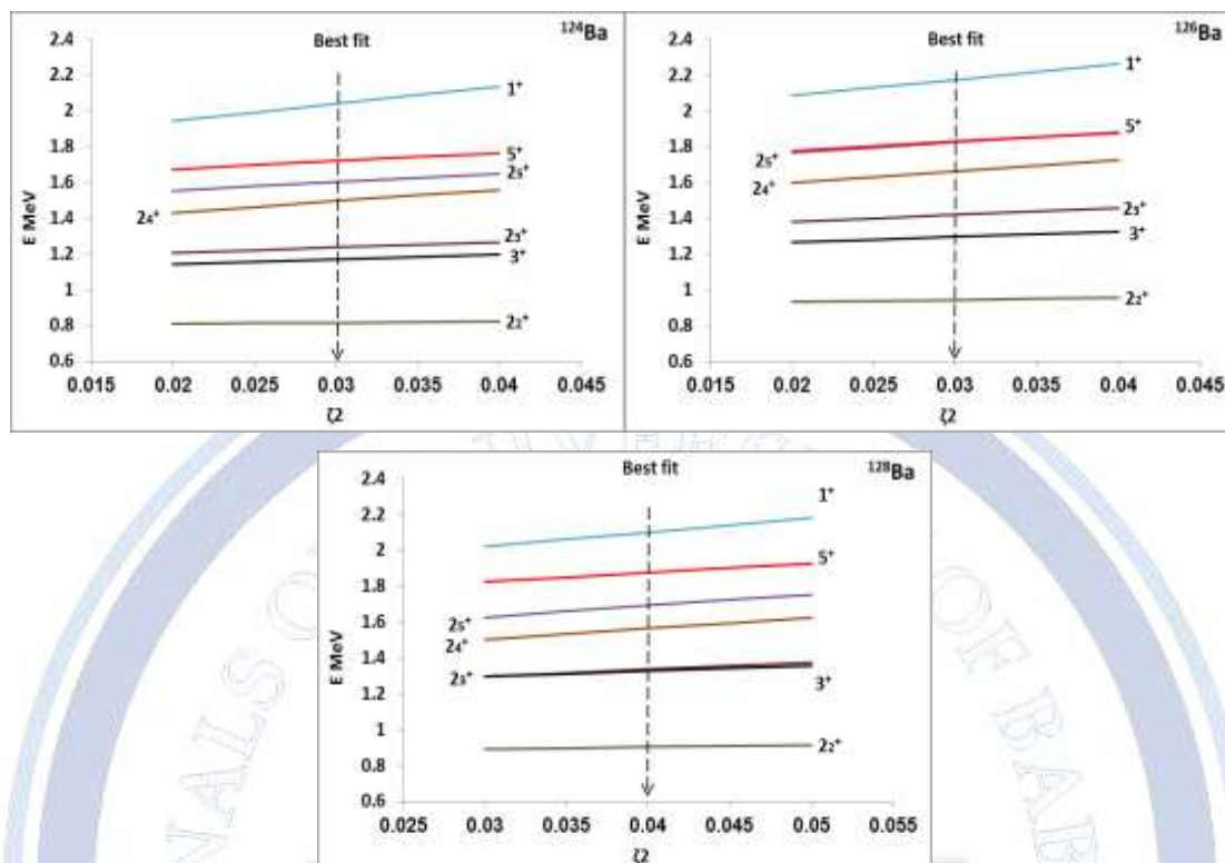
Figure (5) Mixed symmetry states (MSS) in even- even ^{124-128}\text{Ba} isotopes.
