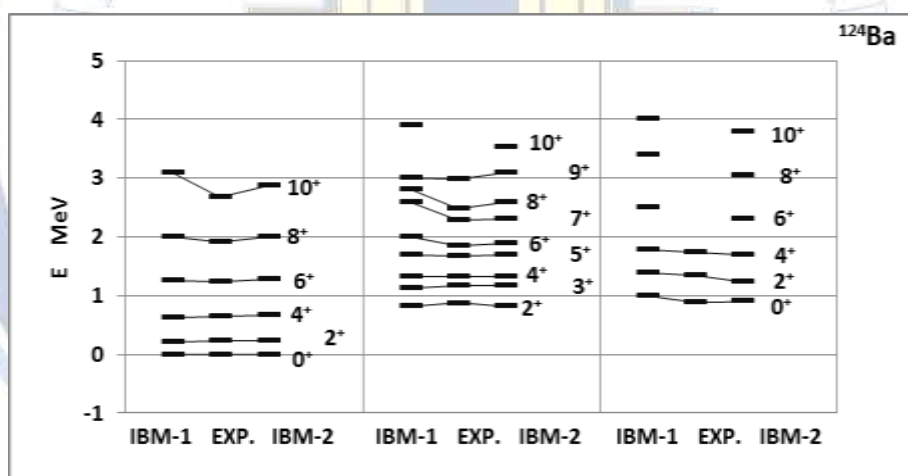
Figure 2: Comparison between experimental [34] and calculated energy levels for ^{124}\text{Ba} isotope.
