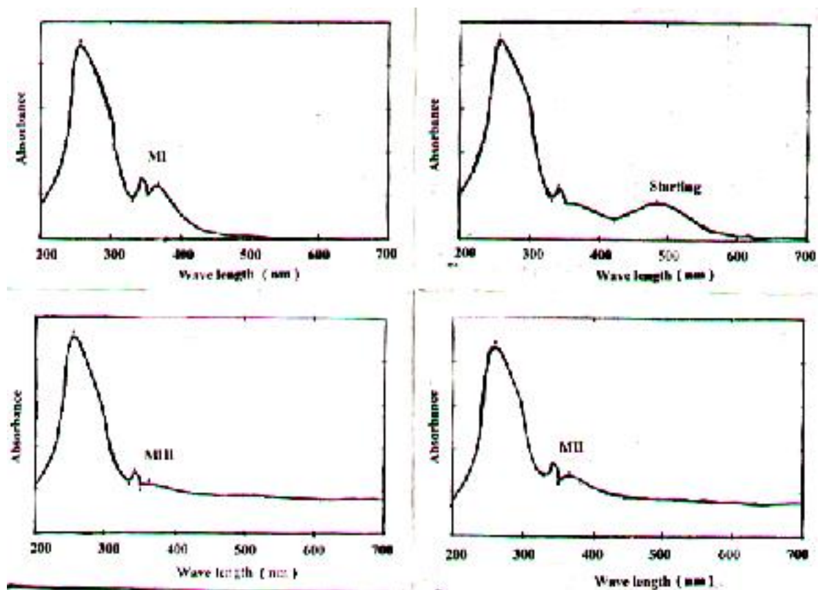
Fig. (3): Absorption spectra of Mo(CO) 4 bipy and their complexes in chloroform solvent
