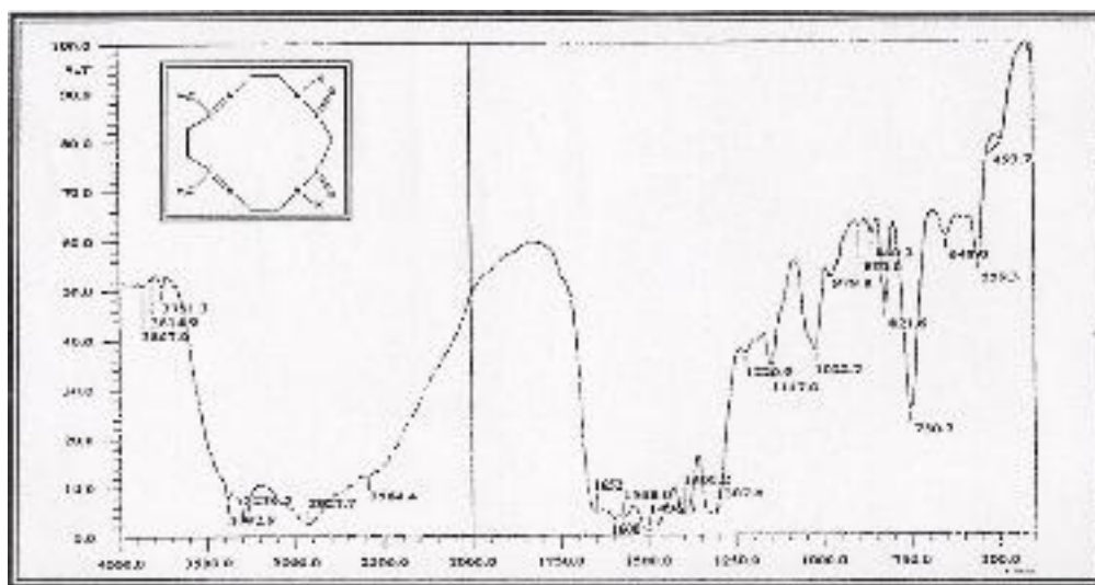
Fig.(2): I.R. Spectrum of the Ligand [H_2L] .
