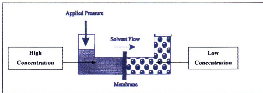
Figure (1): Reverse Osmosis process.
