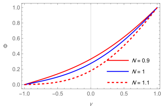
Figure 25: concentration profile with different values N , with \omega = 1, n = 0.1, Q = 0.8, Pe = 0.2, K_r = 0.1, S_r = 0.5, S_c = 0.3, i = \sqrt{-1}, t = 0.5
