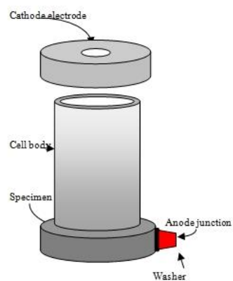
Fig. (1) Electrochemical cell for deposition of nanowires.
