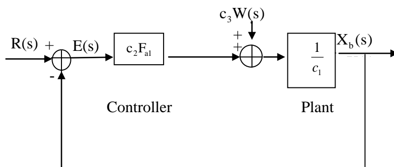
Figure (2). Block Diagram of System (Eq.10)
