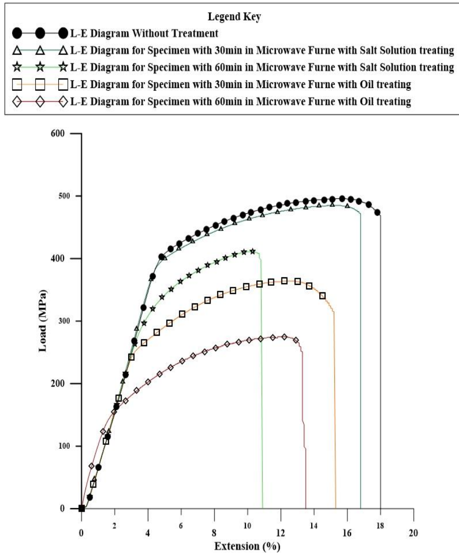
Figure (9): Stress – Strain chart for tensile test of all tests samples
