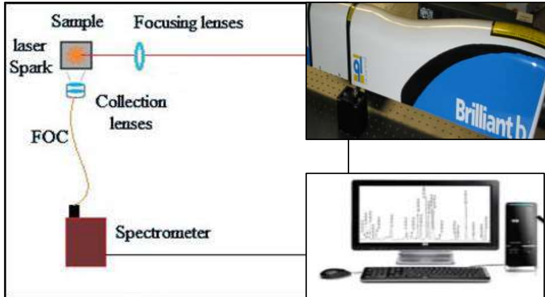
Fig 1: laser induced breakdown spectroscopy diagram of test
