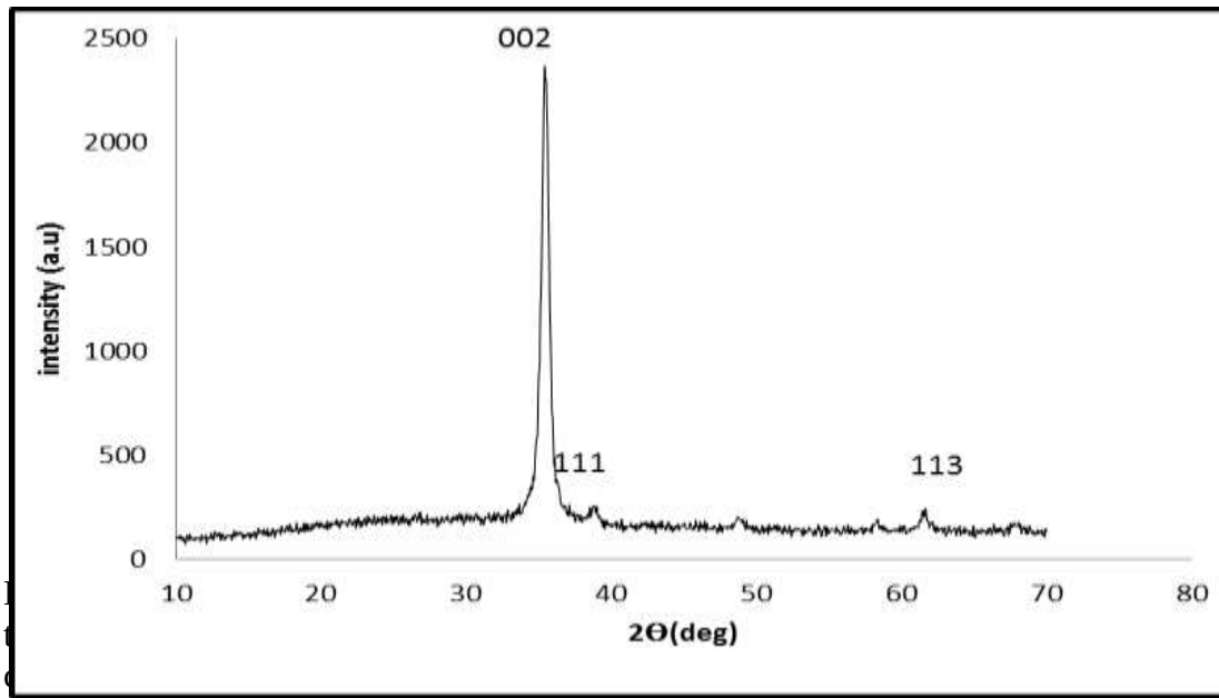
Figure 2: the XRD of Cu Nanoparticles
