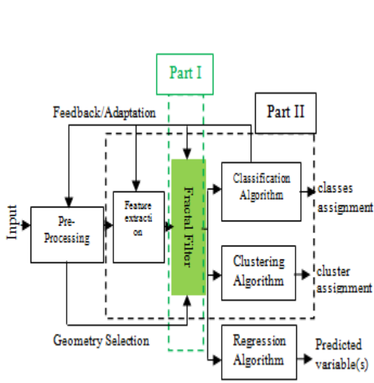
Figure 4. Block diagram of a proposed fractal based pattern recognition system
