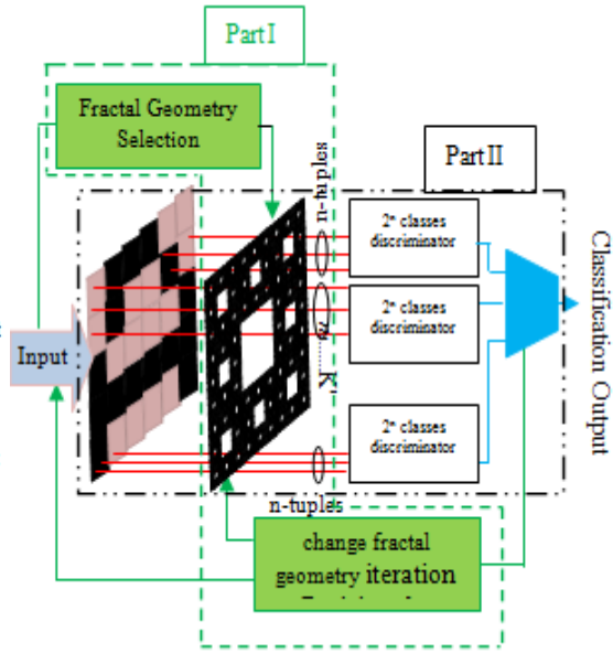
Figure 5. Operation of the proposed fractal-based pattern recognition system
