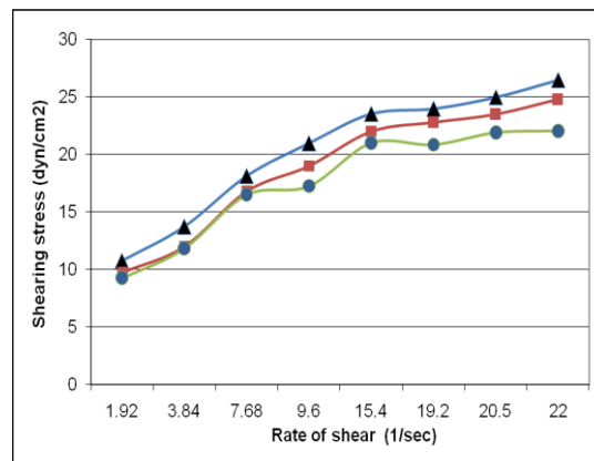
Figure 5 : Rheological behavior of the suspensions , of the extracted L.royleana mucilage ,1.5 % ( w/v ) (▲), chitosan 1.5 % (w/v) (■) and xanthan gum 0.35% (■).
