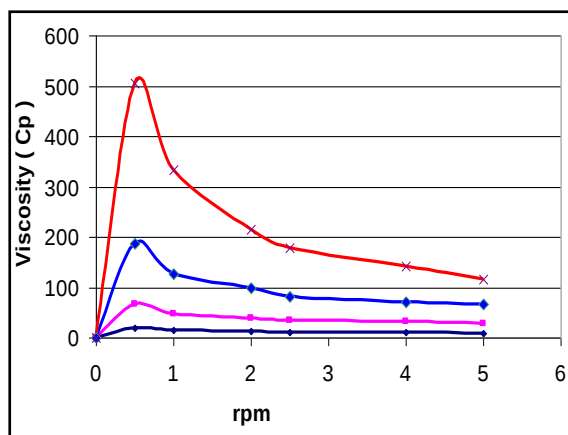
Figure 1 : Comparative evaluation of viscosity of the extracted L.royleana mucilage (—x—), chitosan (—■—), the synthetic polymers carbopol 934 (—■—) and HPMC (—■—). Using 1% w/v solution at 30^{\circ}\text{C} \pm 1 . Values are expressed as the mean of 6 observations. speed of viscometer ; rpm(round per minute)
