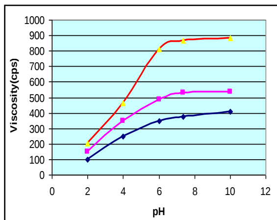
Figure 3 : Effect of pH on viscosity of various concentrations of the extracted L.royleana mucilage. (—◆—) 0.5%, (—■—) 1%, (—▲—) 3% w/v .
