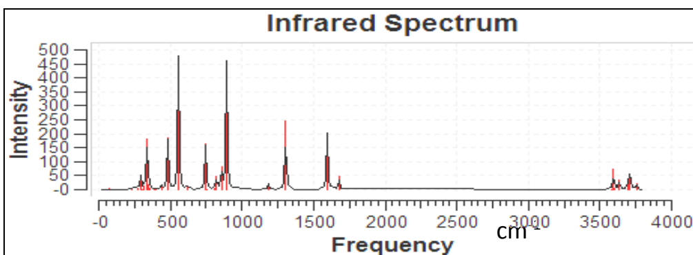
Figure(3-7): IR spectrum for 64 atoms (core & surface)
