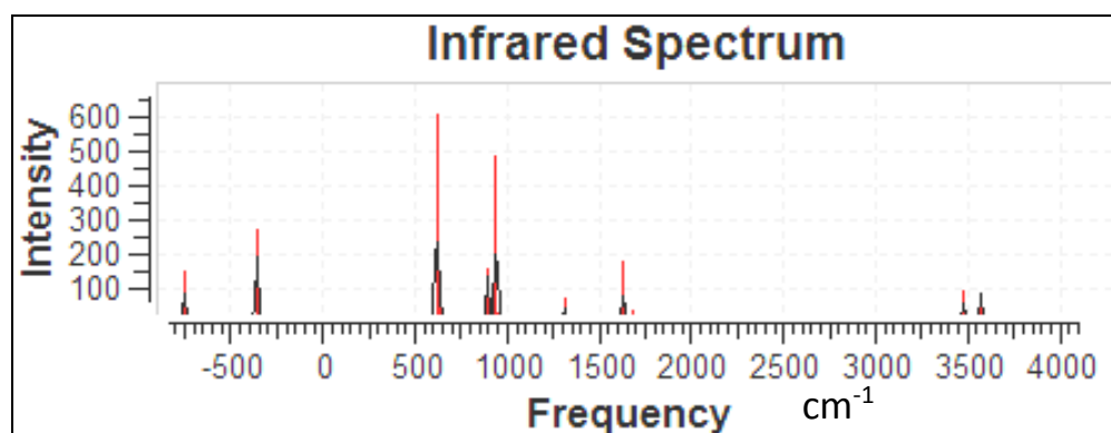
Figure(3-5): IR spectrum for 128 atoms (core)
