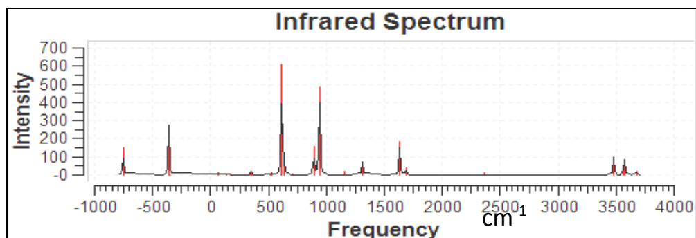
Figure(3-6): IR spectrum for 8 atoms (core & surface)
