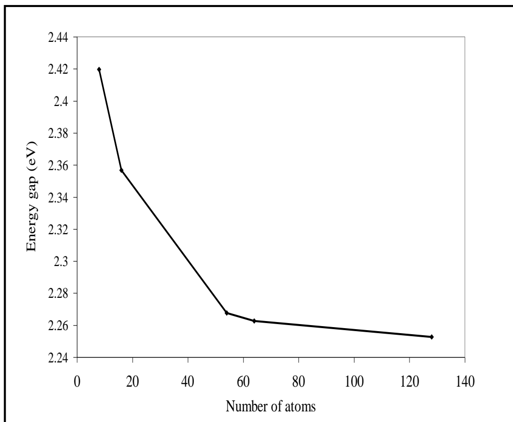
Fig. (1) The energy gap of germanium core nanocrystals as a function of number of atoms.
