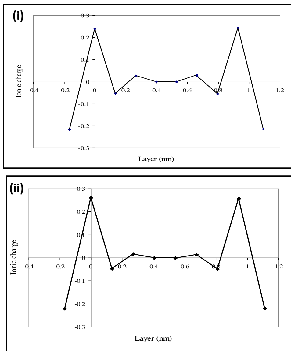
Fig.(2) the Ionic charge for the two oxygenated surface [(a) a^2 (b) 4a^2 ] area .
