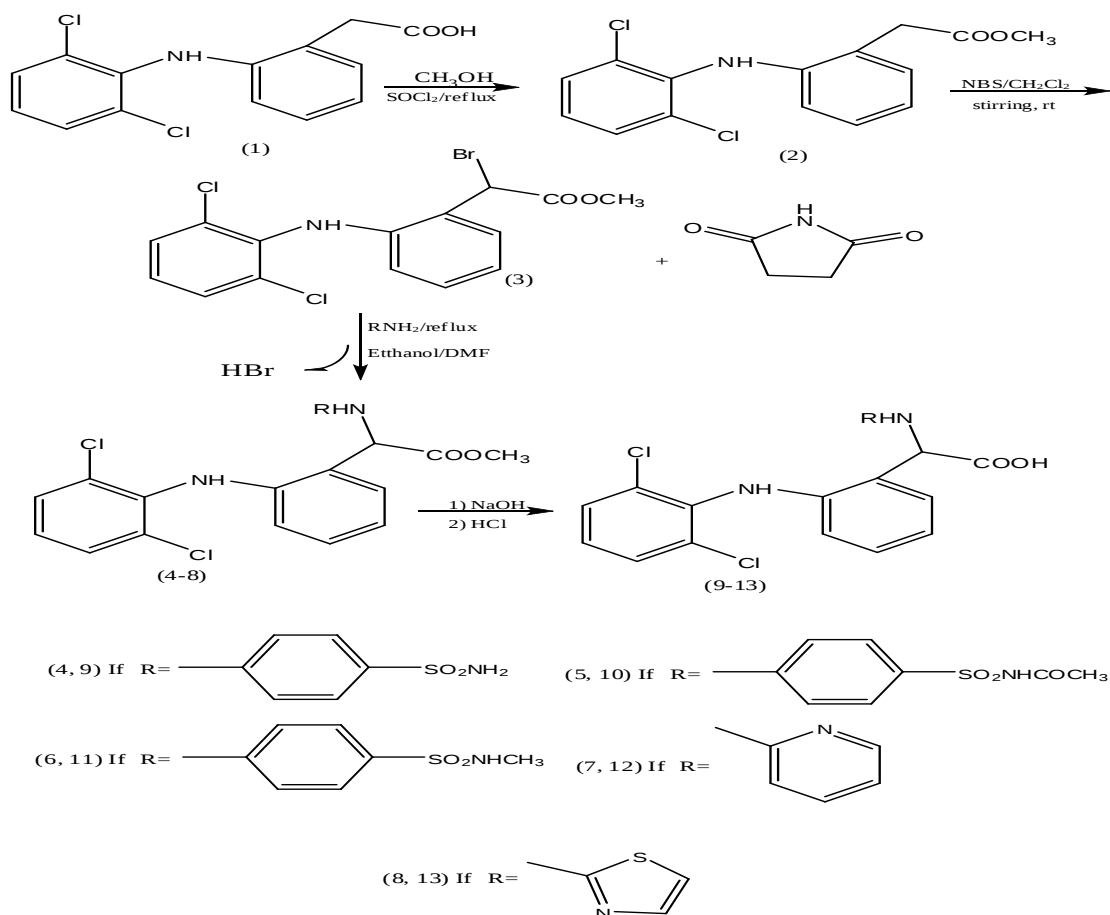
Scheme1: Synthesis of target compounds (9-13) and their intermediates.
