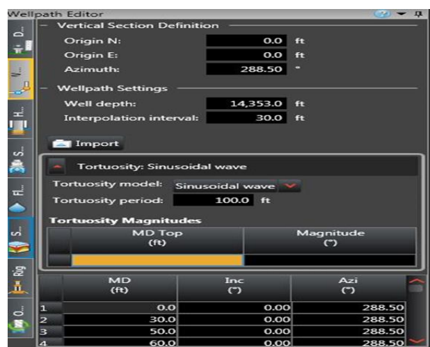
Fig. 7. Well path information for ZB-250
