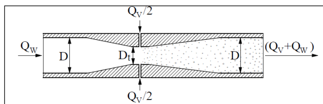
Fig. 1 Venturi tube induced air suction [3].
