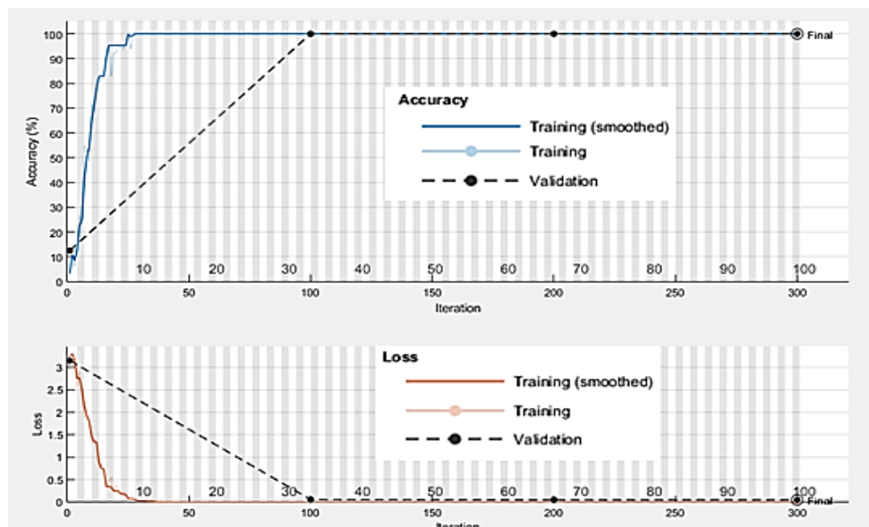
Figure 17: Accuracy and loss functions results
