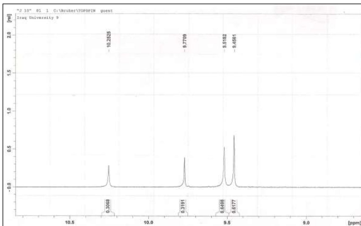
Fig. 11: 1 H -NMR spectrum of compound [9]
