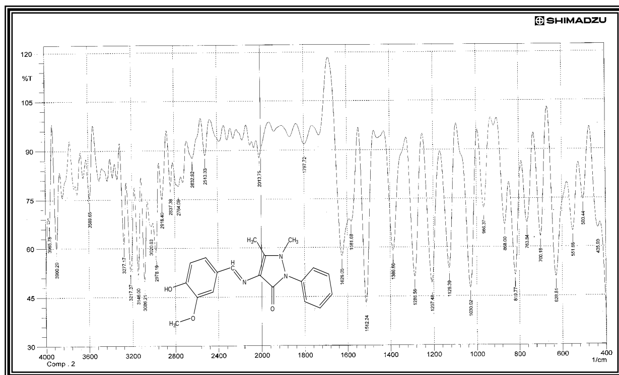
Fig. 3: FT-IR spectrum of compound [2]
