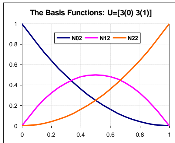
Figure2. Basis function: U = [0(3) \ 1(3)]
