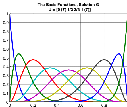
Figure 14. Basis function: U = [0(7) 1/3 2/3 1(7)]
