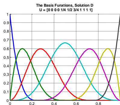
Figure 8. Basis function:
