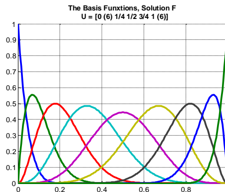
Figure 12. Basis function: U = [0(6) \ 1/4 \ 1/2 \ 3/4 \ 1(6)]
