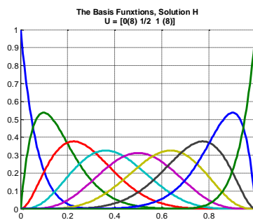
Figure 16. Basis function: U = [0(8) \ 1/2 \ 1(8)]
