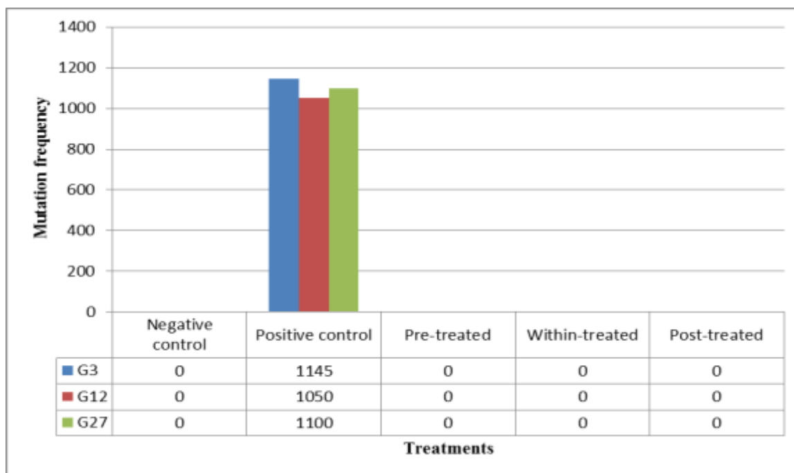
Figure (3): The effect of the interaction between the optimum concentration of C. colocynthis seed alcoholic extract and MTX to induce mutations of G-system isolates.
