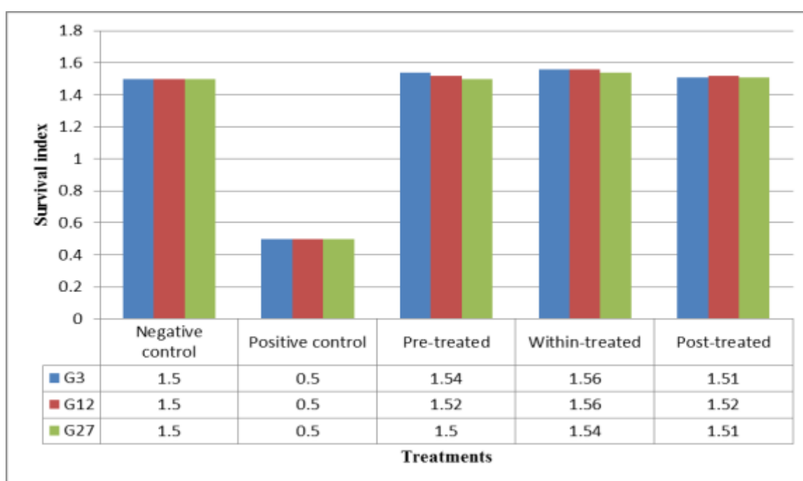
Figure (4): The effect of the interaction between the optimum concentration of C. colocynthis seed alcoholic extract and exposure to UV on the survival index of G-system isolates.
