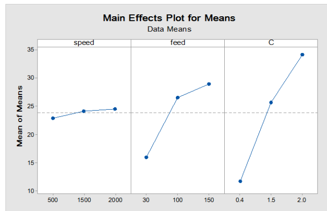
Figure 3: Main effect plot for MRR
