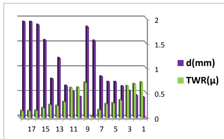
Figure 11: The influence of depth of cut on TWR
