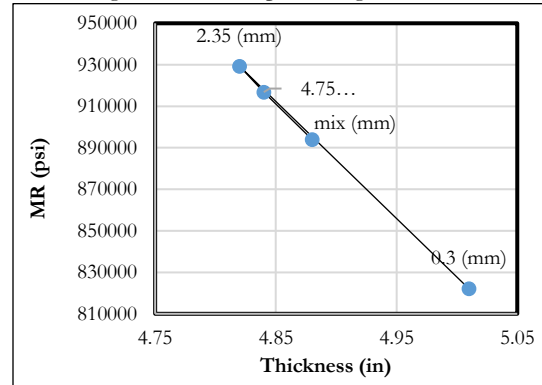
Figure (13): The relationship between binder layer thickness (in) and MR (psi) for CR-asphalt mixtures with different gradations and 1% of CR.
