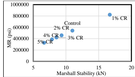
Figure (6): the relationship between Marshall Stability and Resilience Modulus (MR) for control and CR-modified asphalt mixture with 0.3mm gradation.
