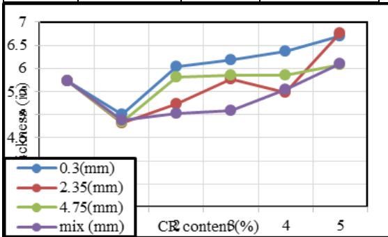
Figure (10): The binder layer thickness (in) for CR-asphalt mixtures with different gradations and percentages of CR.
