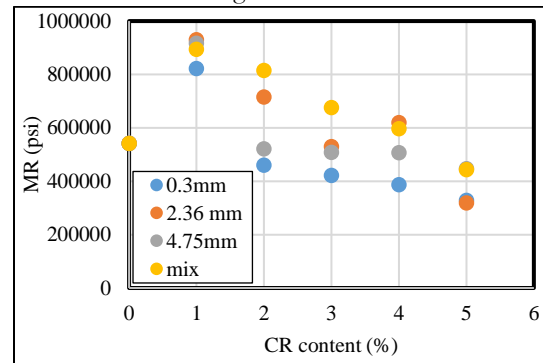
Figure (7): Resilience Modulus (MR) values for control and CR-asphalt mixtures with different gradations and percentages of CR.
