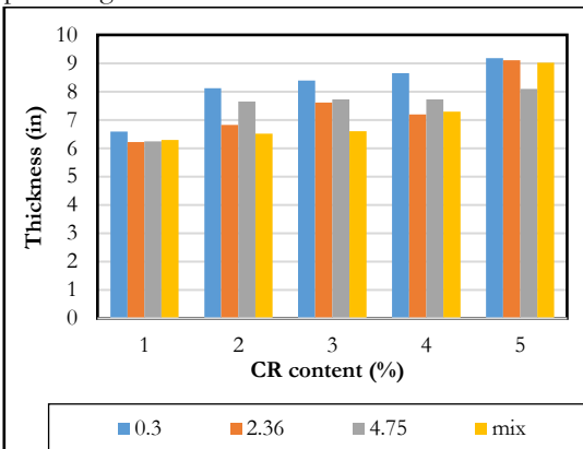
Figure (11): The comparison of binder layer thickness (in) for CR-modified asphalt mixtures with different percentages of CR.
