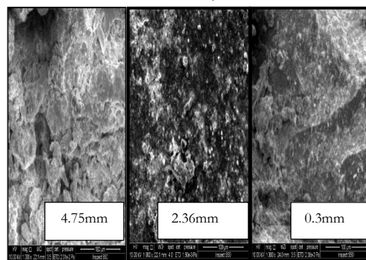
Figure (4): Scanning Electron Microscopy results of crumb rubber (CR) with different sizes at 100 \mu\text{m} .
