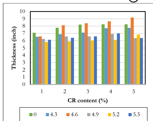
Figure (13): the binder layer thickness of CR-modified asphalt mixtures with different asphalt binder contents and percent of CR at gradation of 0.3mm.
