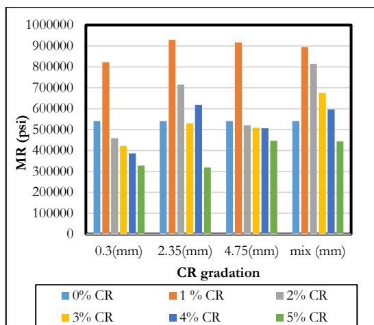
Figure (8): Comparison of Resilience Modulus (MR) between different CR-modified mixtures with different gradations and percentages of CR.
