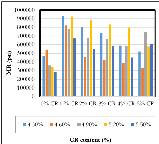
Figure (9): Resilience Modulus (MR) of CR-modified asphalt mixtures with different asphalt binder contents and percent of CR at gradation of 0.3mm.
