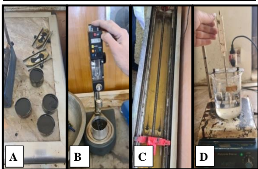
Figure (2): Physical Properties Tests for Asphalt binder, A- preparing the samples, B- penetration test, C- Ductility, D- Softening Point.
