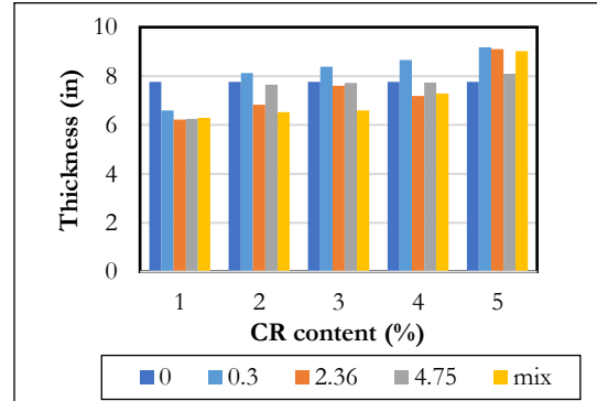
Figure (12): Comparison of binder layer thickness between different CR-modified mixtures with different gradations and percentages of CR.
