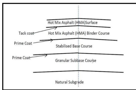
Figure(5): Typical flexible pavement configuration: High Traffic Volume (Congress, I. R., 2001)
