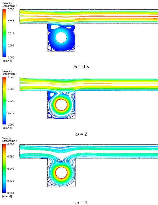
Fig. 12 Streamlines contour at Re = 100 , Ri = 1 .
