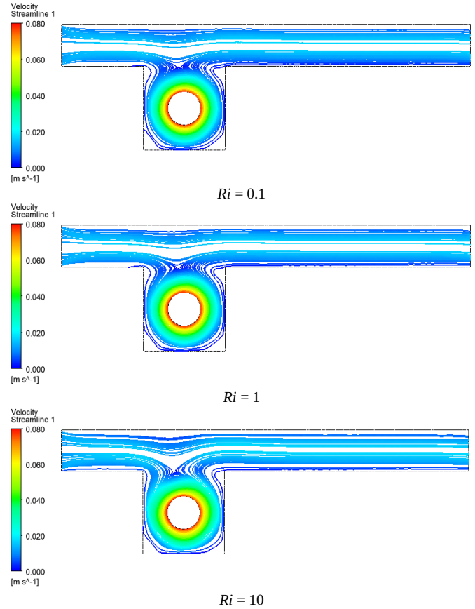
Fig. 4 Streamlines contours at Re = 50 , \omega = 4 rad/sec.
