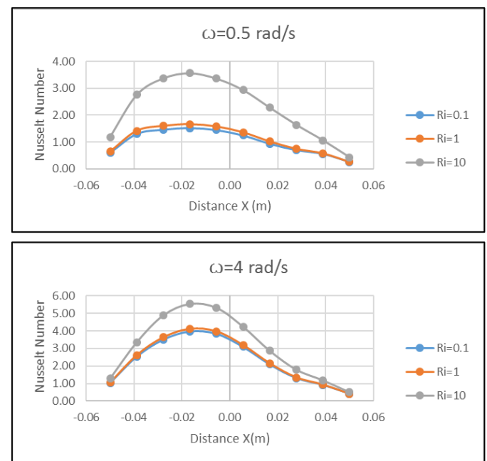
Fig. 14 Variation of Nusselt number along the heated surface at Re = 50 .
