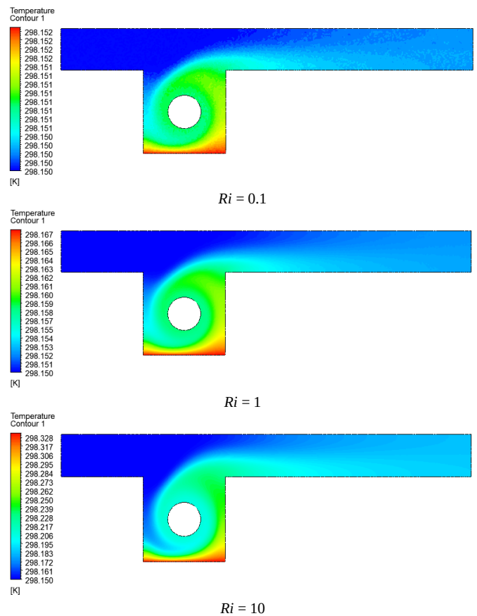
Fig. 4 Isothermal contours at Re = 50 , \omega = 4 rad/sec.
