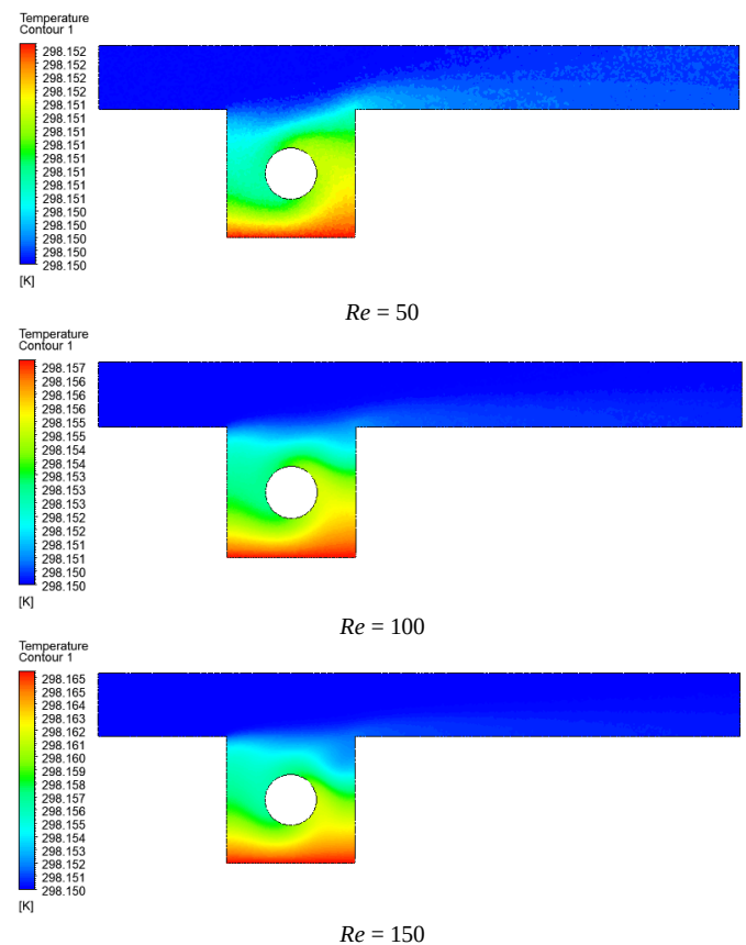
Fig. 7 Isothermal contours at Ri = 0.1 , \omega = 0.5 rad/sec.
