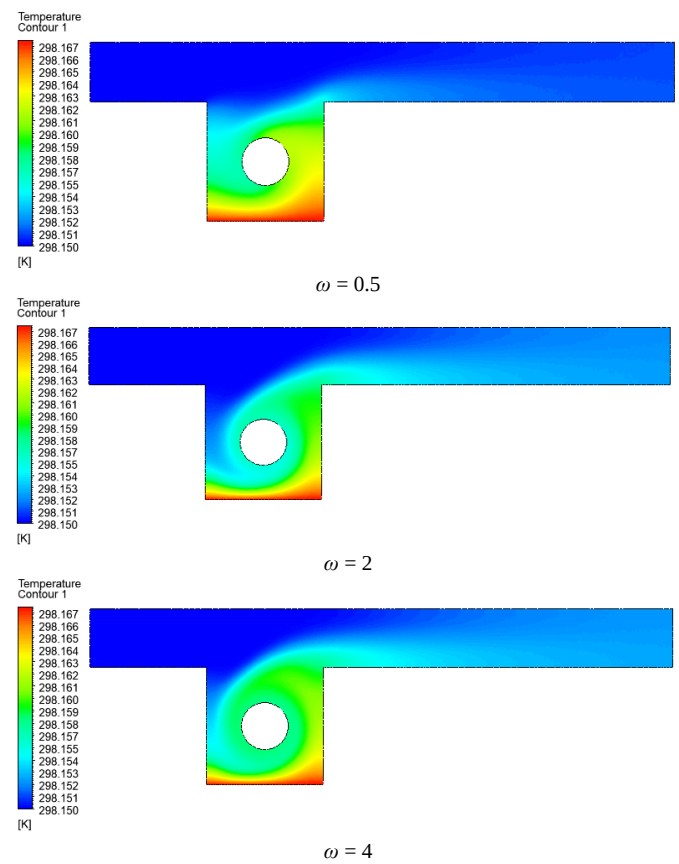
Fig. 11 Isothermal contours at Ri = 1 , Re = 50 .
