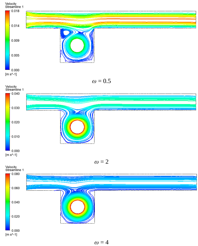
Fig. 10 Streamlines contour at Ri = 1 , Re = 50 .
