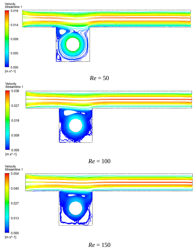
Fig. 6 Streamlines contours at Ri = 0.1 , \omega = 0.5 rad/sec.
