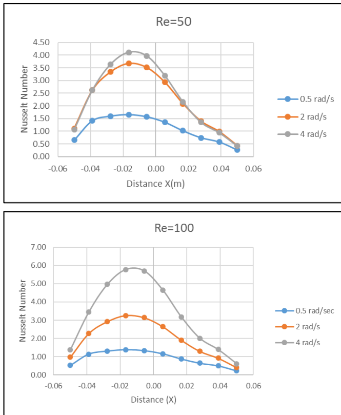
Fig. 16 Variation of Nusselt number along the heated surface at Ri = 1 .
