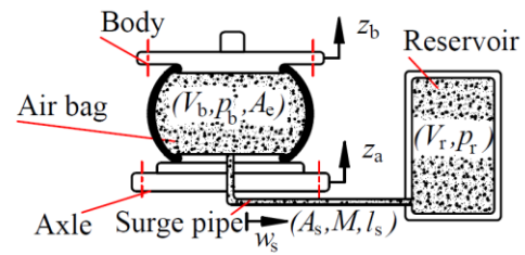
Fig. 2 Structure schematic of Gensys [16].
