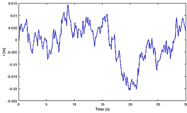
Fig. 5 Roughness road input profile ISO class B.
