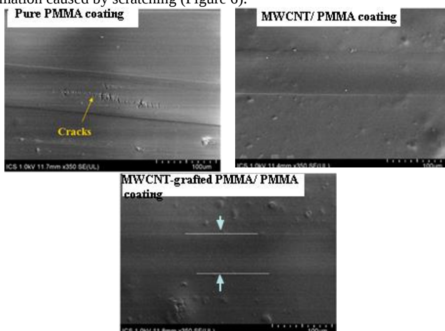
Figure 6 SEM micrographs of the worn surface
