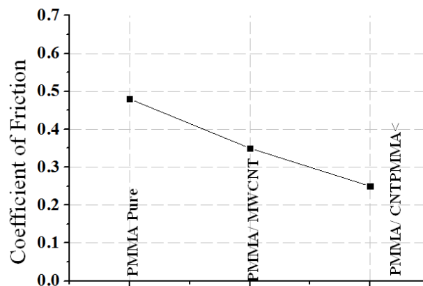
Figure 5 coefficient of friction for PMMA reinforced with pristine MWCNT and MWCNT grafted PMMA.
