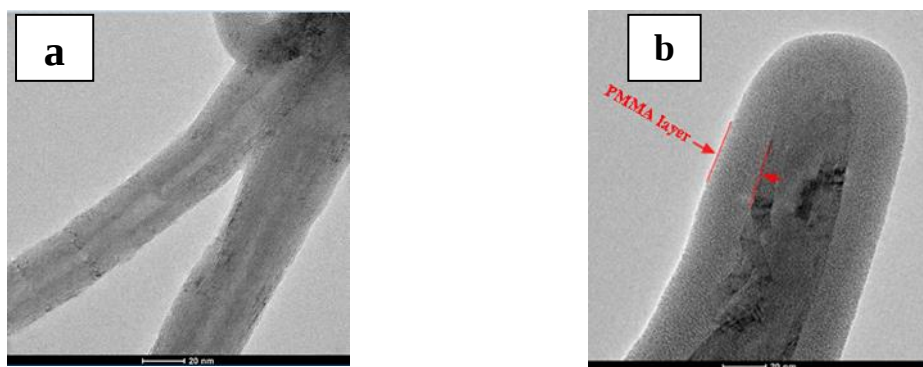
Figure 1 Transmission Electron Microscopy of (a) MWCNT and (b) MWCNT-grafted-PMMA dispersed in THF
