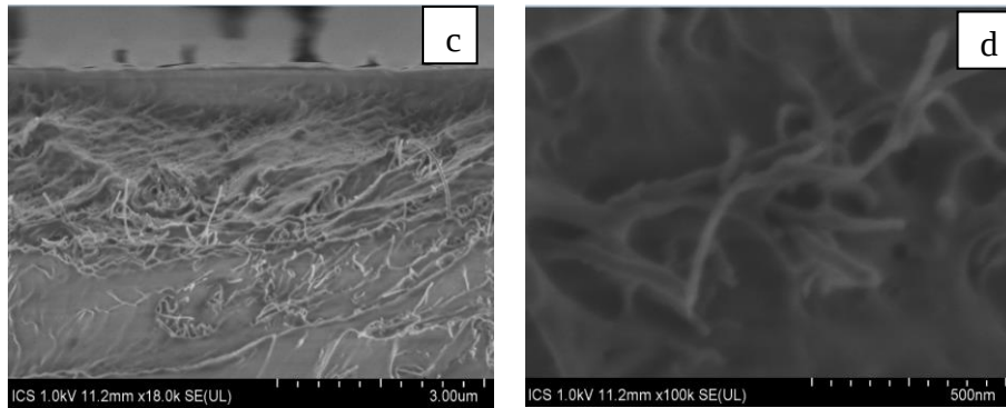
Figure 2 SEM images of a fracture surface of PMMA / MWCNT coating sample
