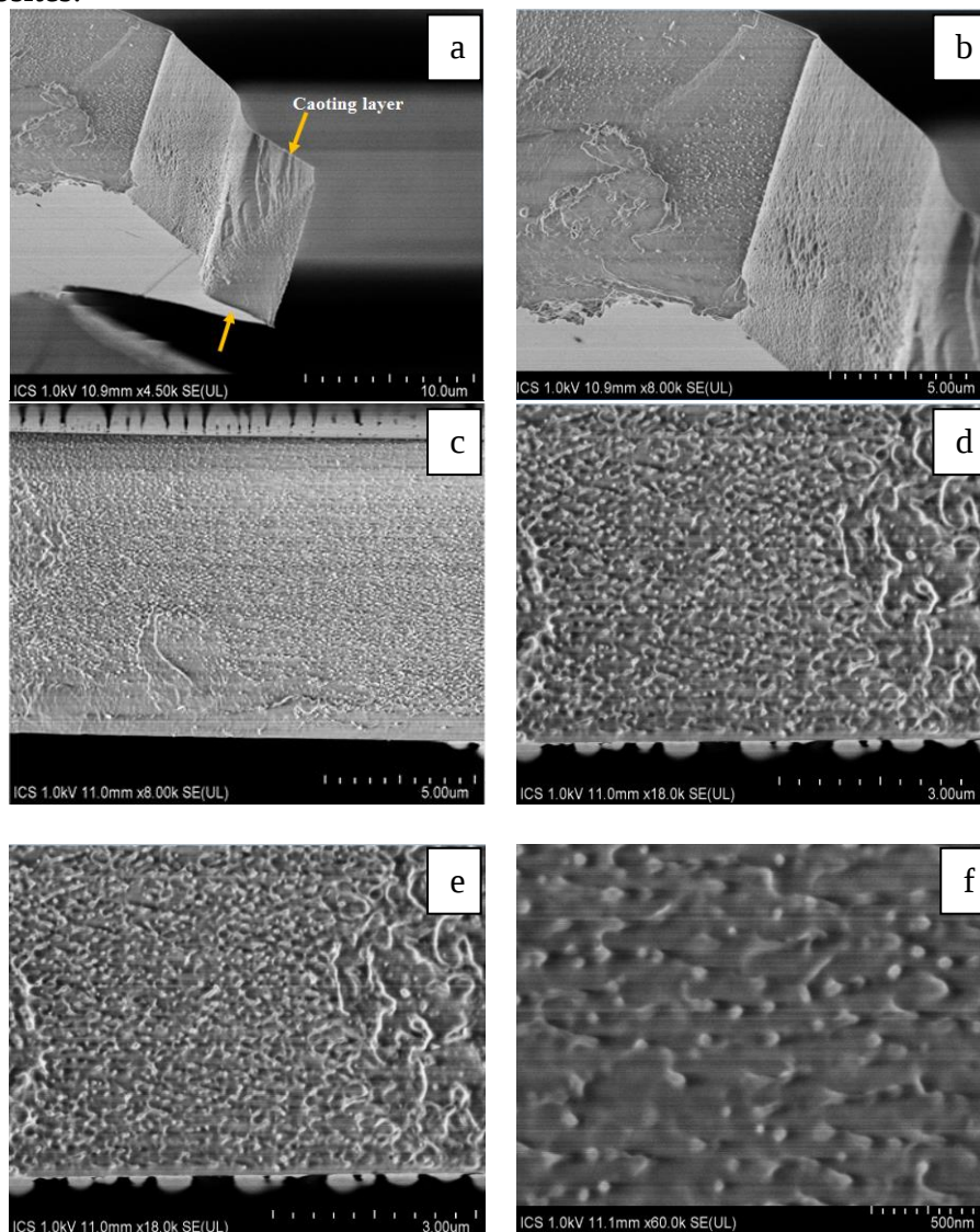
Figure 3 SEM images of a fracture surface of PMMA/CNT sample Hardness & Elastic Modulus
