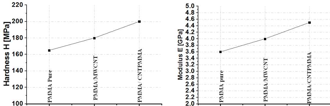
Figure 4 Young's modulus (on the right) and of hardness (on the left)
