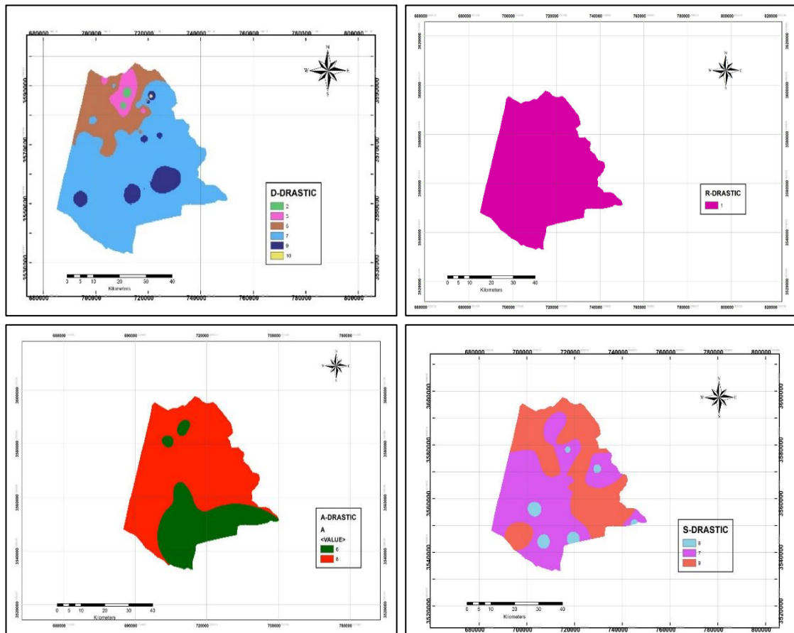
Fig. 2 the rating map of D, R, A, S used in DRASTIC method.
