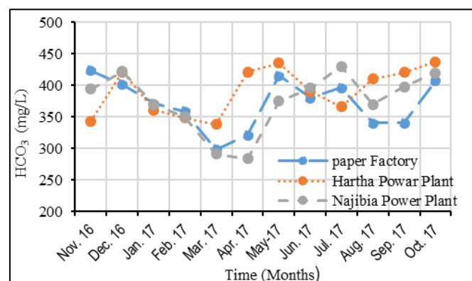
Fig. 3 The amount of HCO 3 concentration in industrial water.
